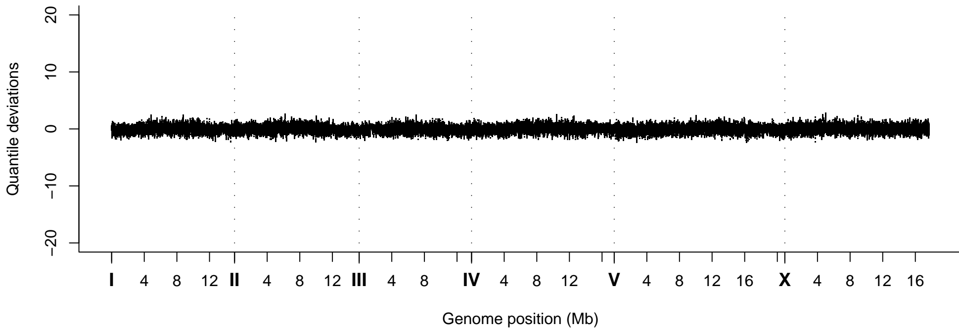
Quantile Deviations, Strain VC20421
