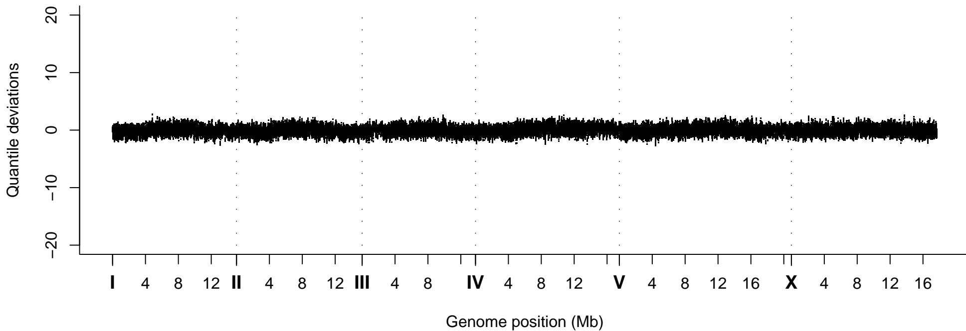
Quantile Deviations, Strain VC20424
