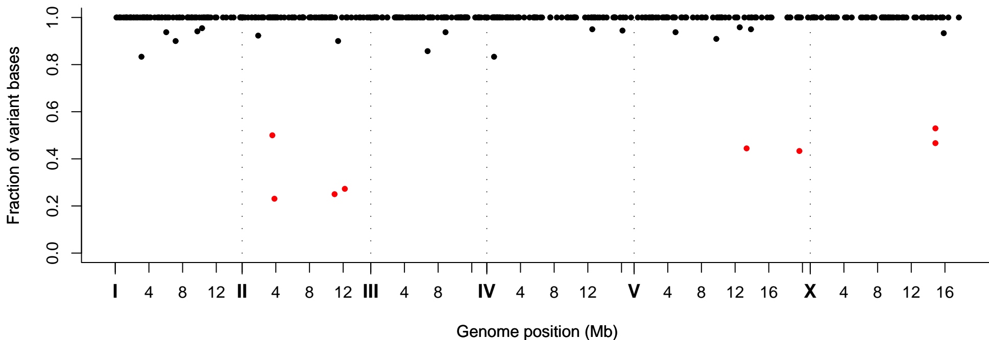
Fraction of Variant Bases at Position, Strain VC20424
