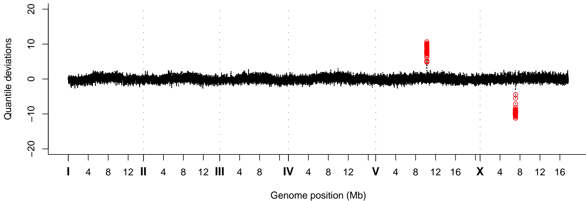
Quantile Deviations, Strain VC20431
