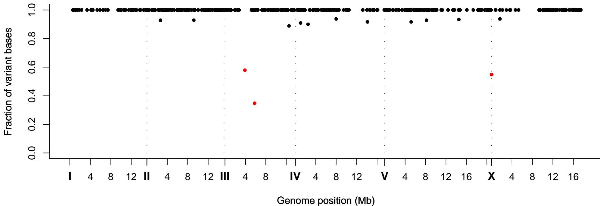
Fraction of Variant Bases at Position, Strain VC20431
