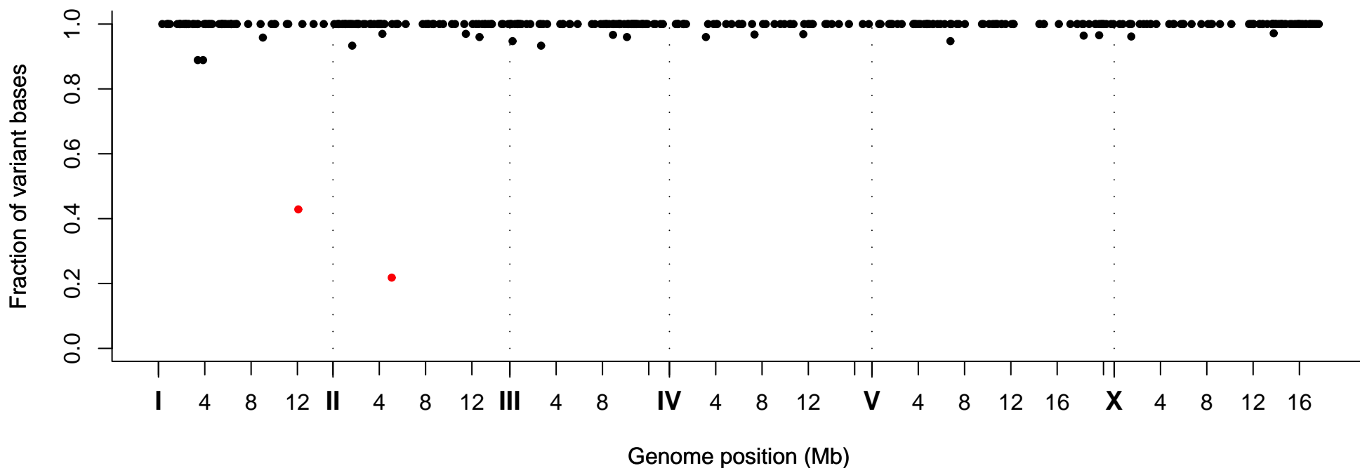
Fraction of Variant Bases at Position, Strain VC20436
