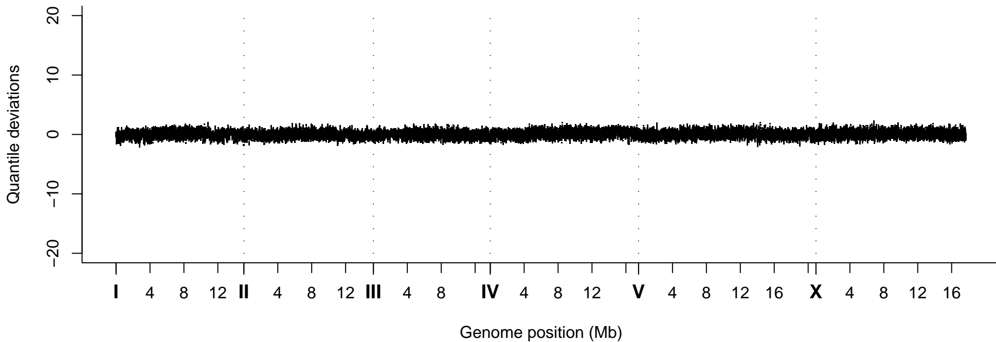
Quantile Deviations, Strain VC20436
