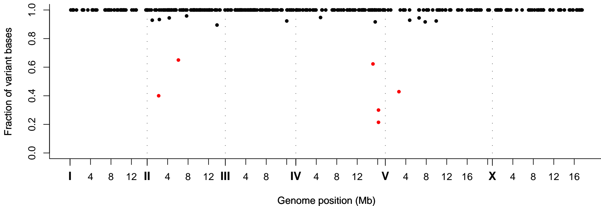
Fraction of Variant Bases at Position, Strain VC20440
