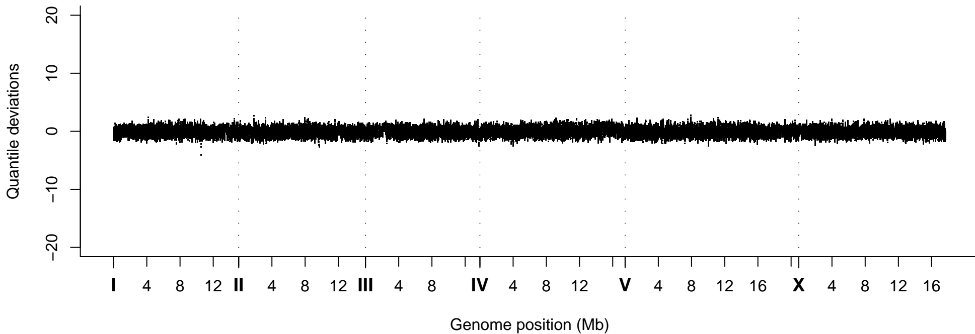
Quantile Deviations, Strain VC20440
