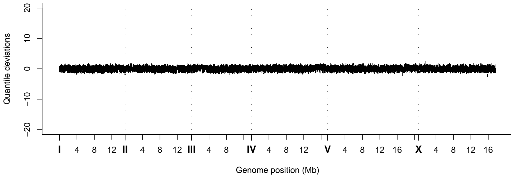
Quantile Deviations, Strain VC20441
