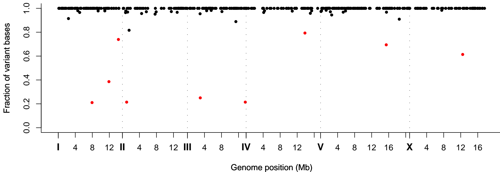
Fraction of Variant Bases at Position, Strain VC20441
