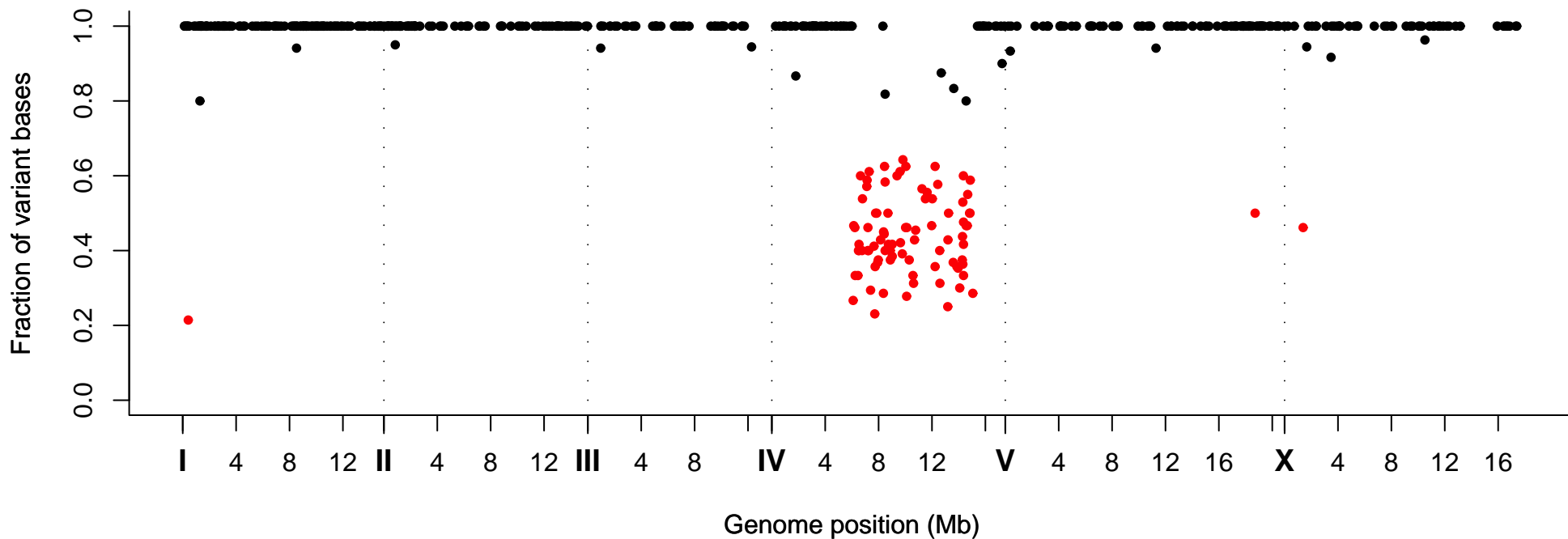
Fraction of Variant Bases at Position, Strain VC20444
