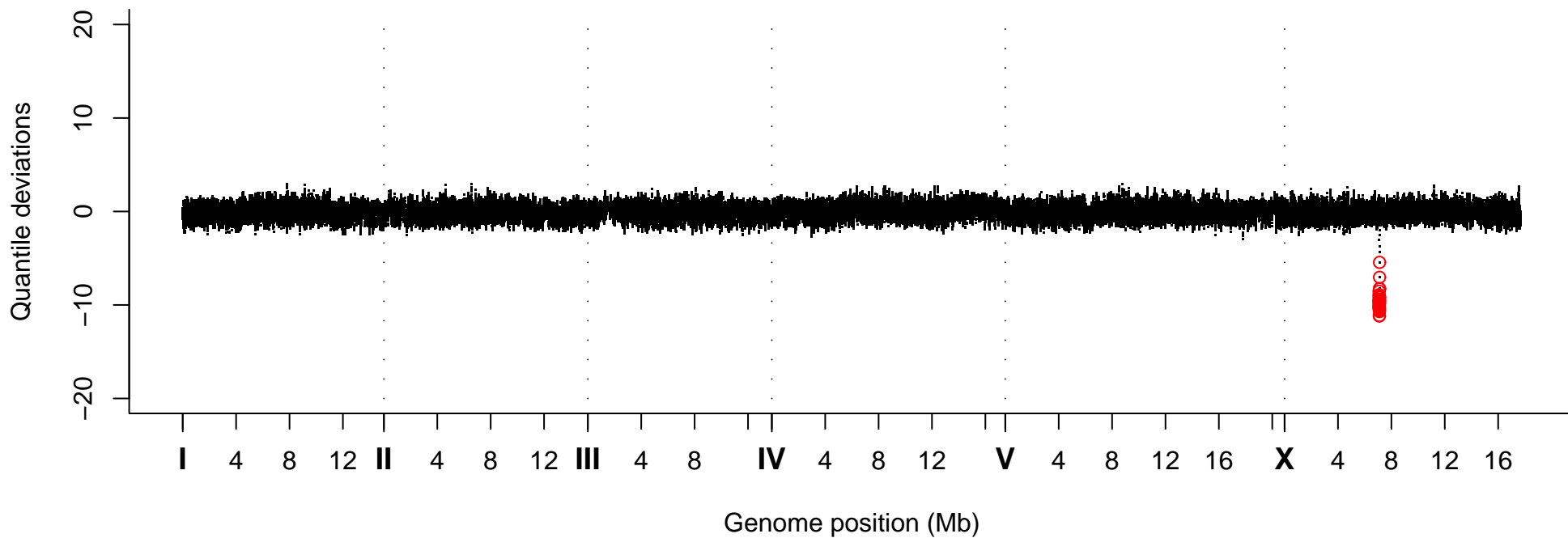
Quantile Deviations, Strain VC20444
