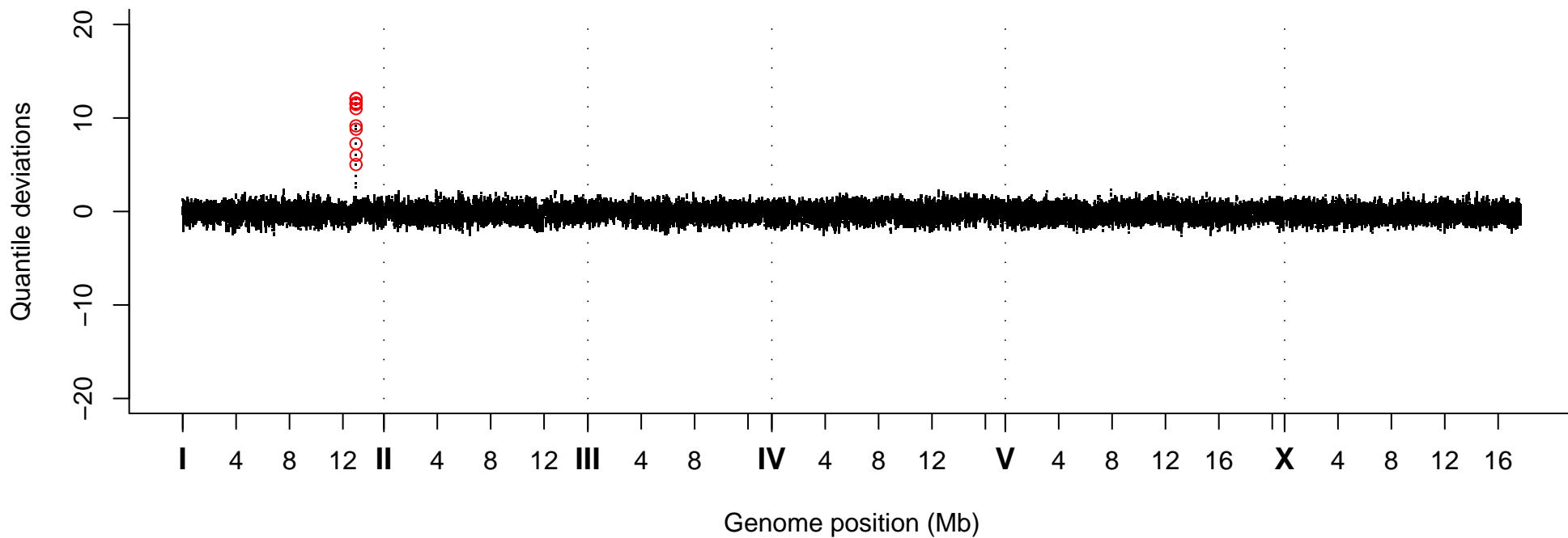
Quantile Deviations, Strain VC20452
