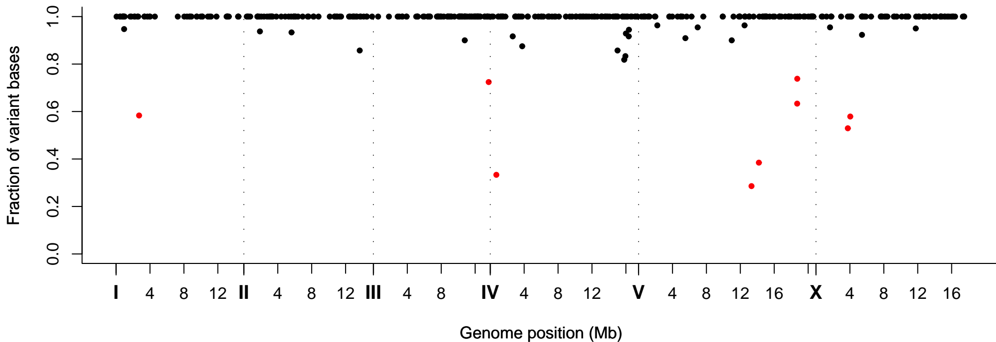
Fraction of Variant Bases at Position, Strain VC20452
