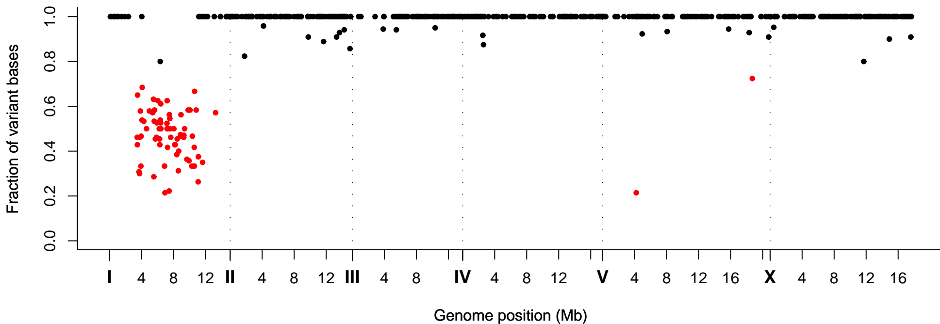
Fraction of Variant Bases at Position, Strain VC20457
