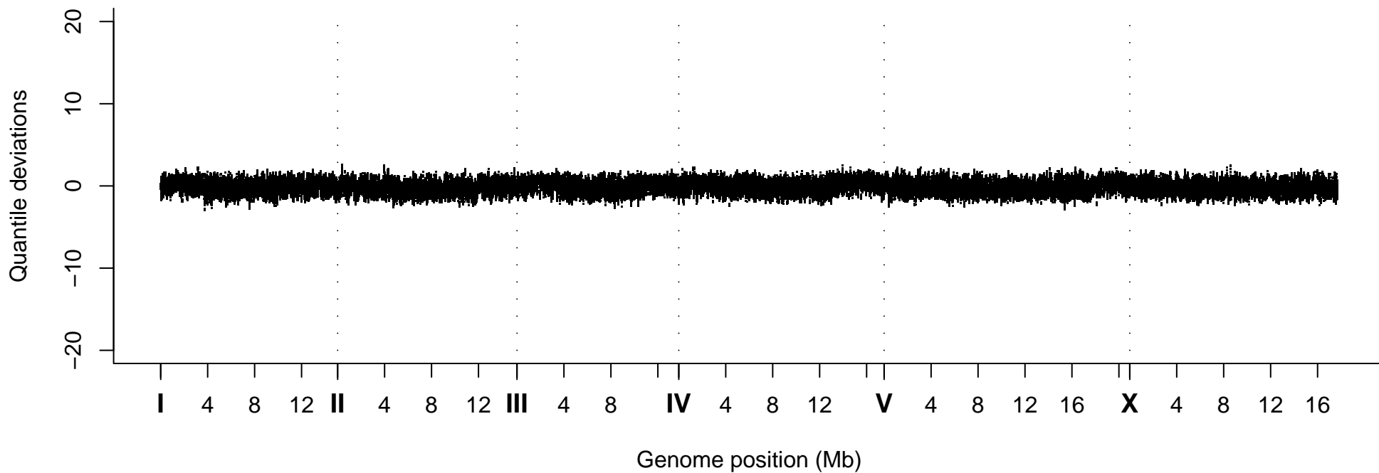
Quantile Deviations, Strain VC20457
