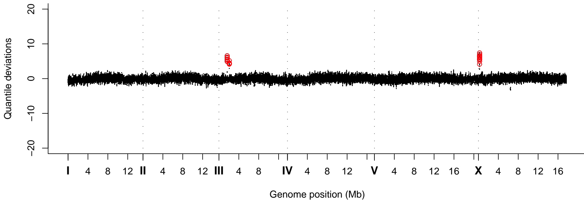
Quantile Deviations, Strain VC20465
