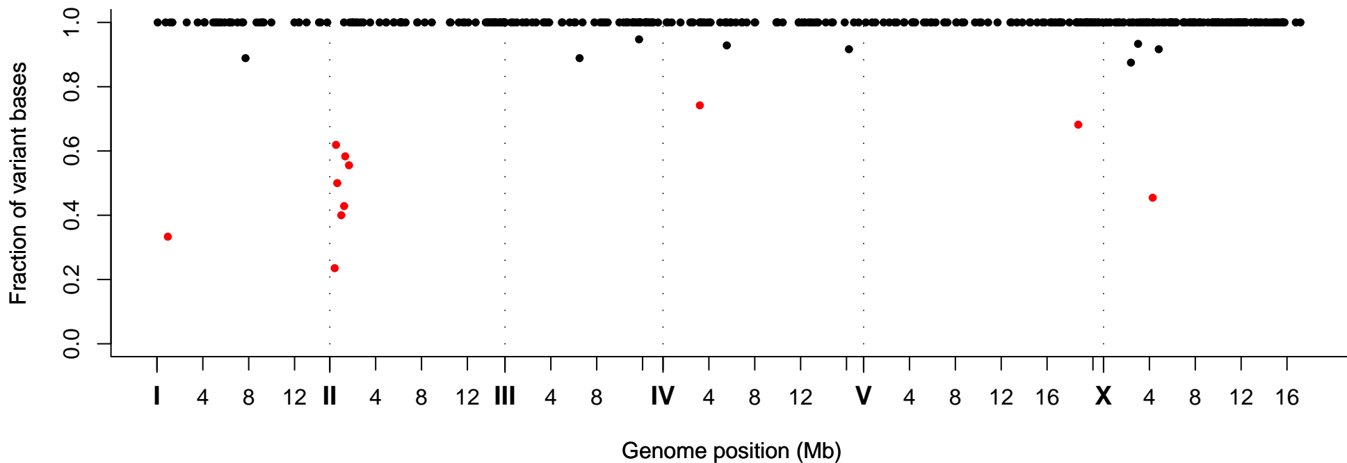
Fraction of Variant Bases at Position, Strain VC20475
