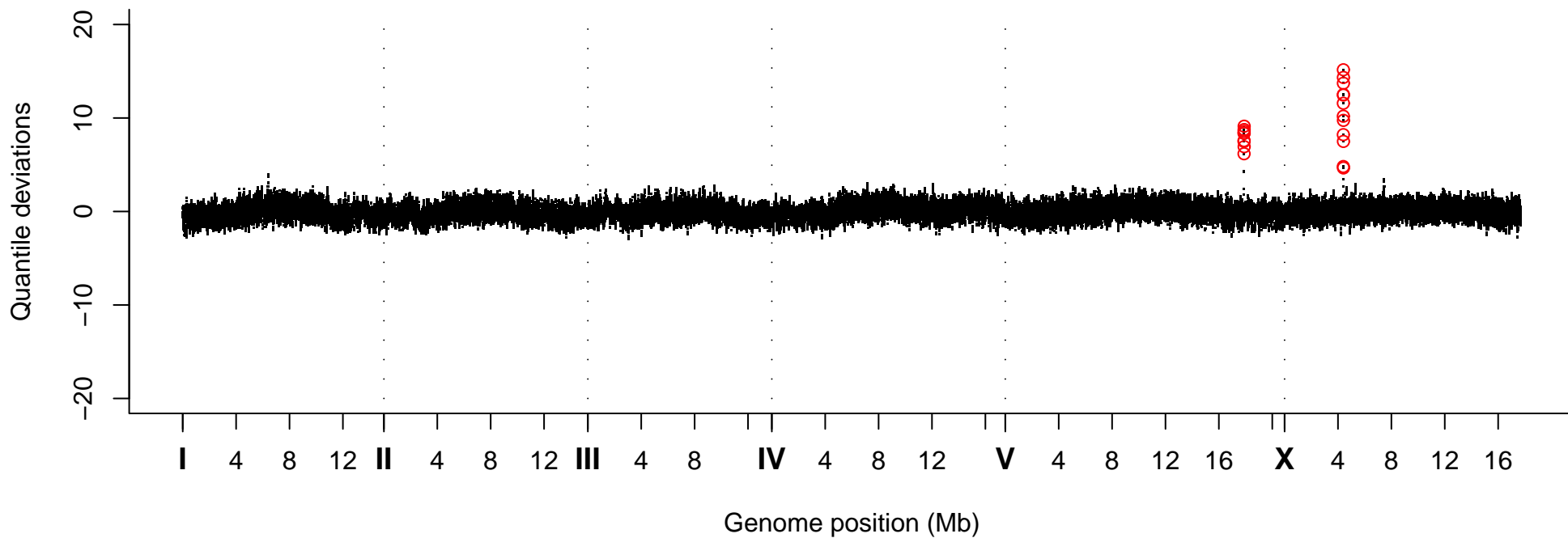
Quantile Deviations, Strain VC20475
