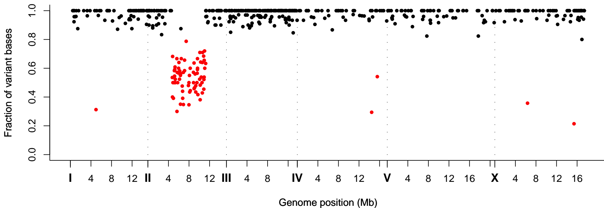
Fraction of Variant Bases at Position, Strain VC20481
