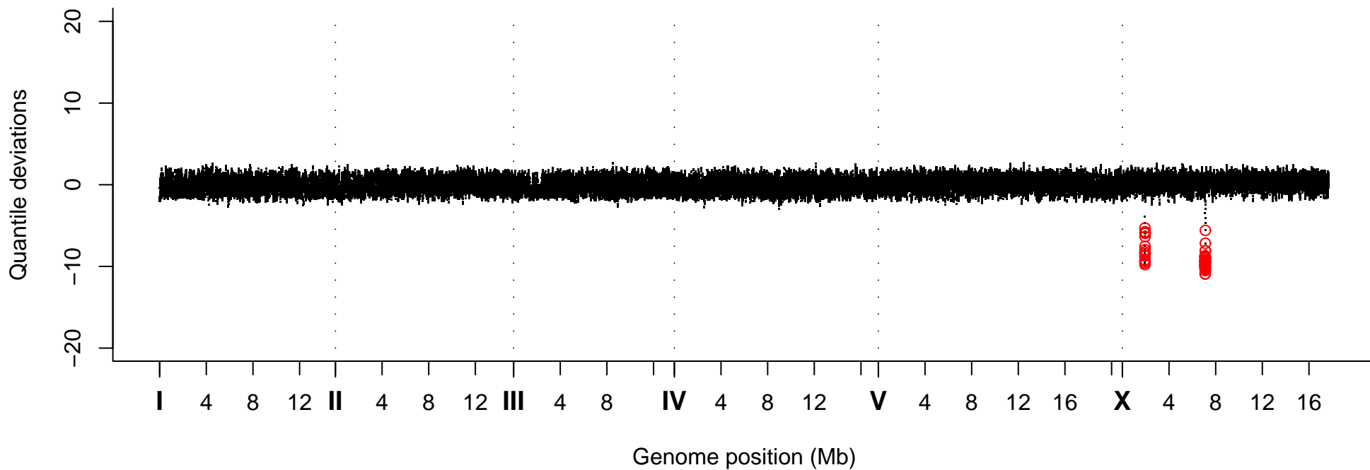
Quantile Deviations, Strain VC20481
