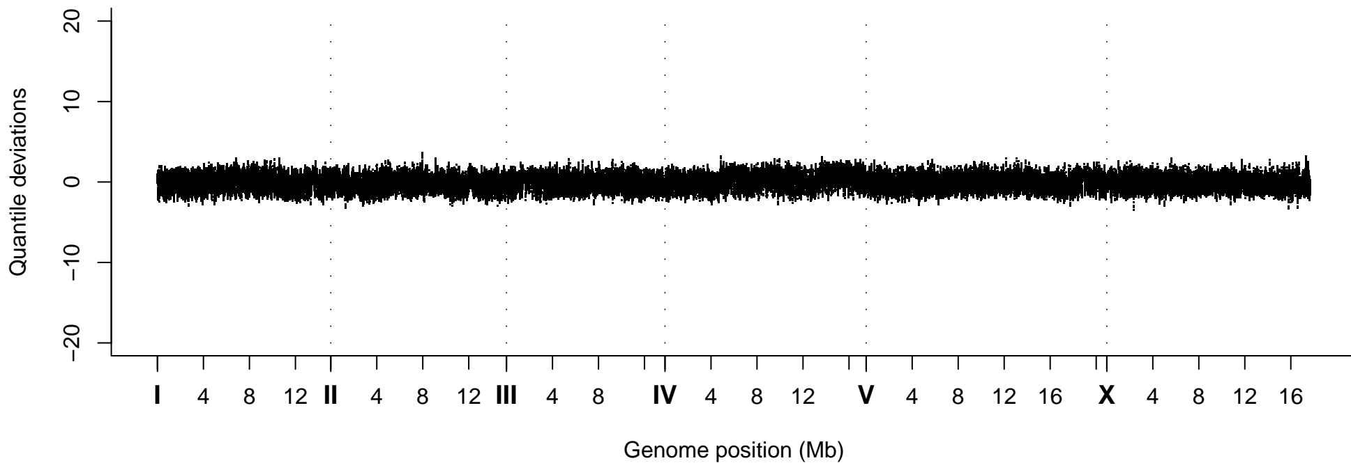
Quantile Deviations, Strain VC20491
