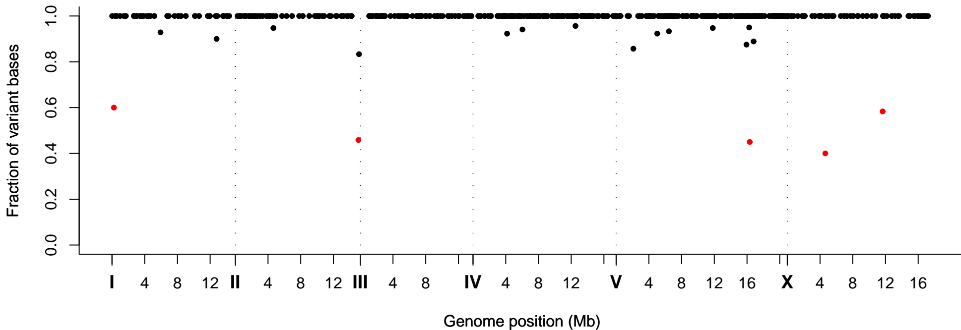
Fraction of Variant Bases at Position, Strain VC20491
