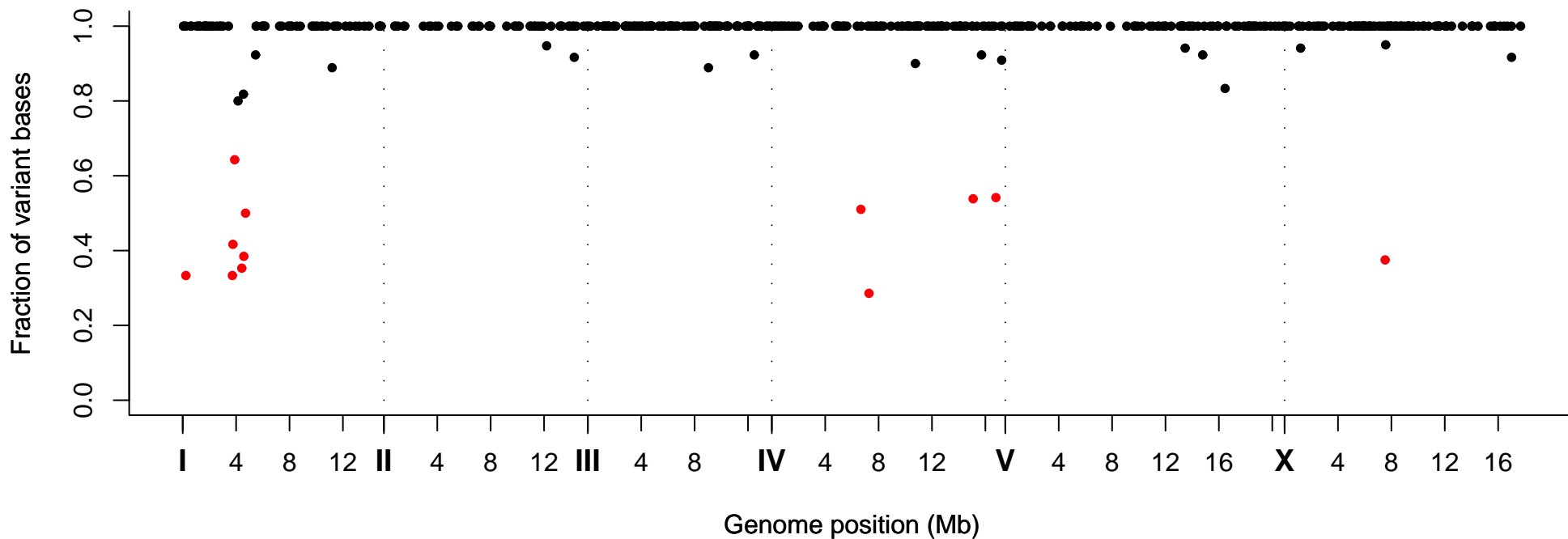
Fraction of Variant Bases at Position, Strain VC20492
