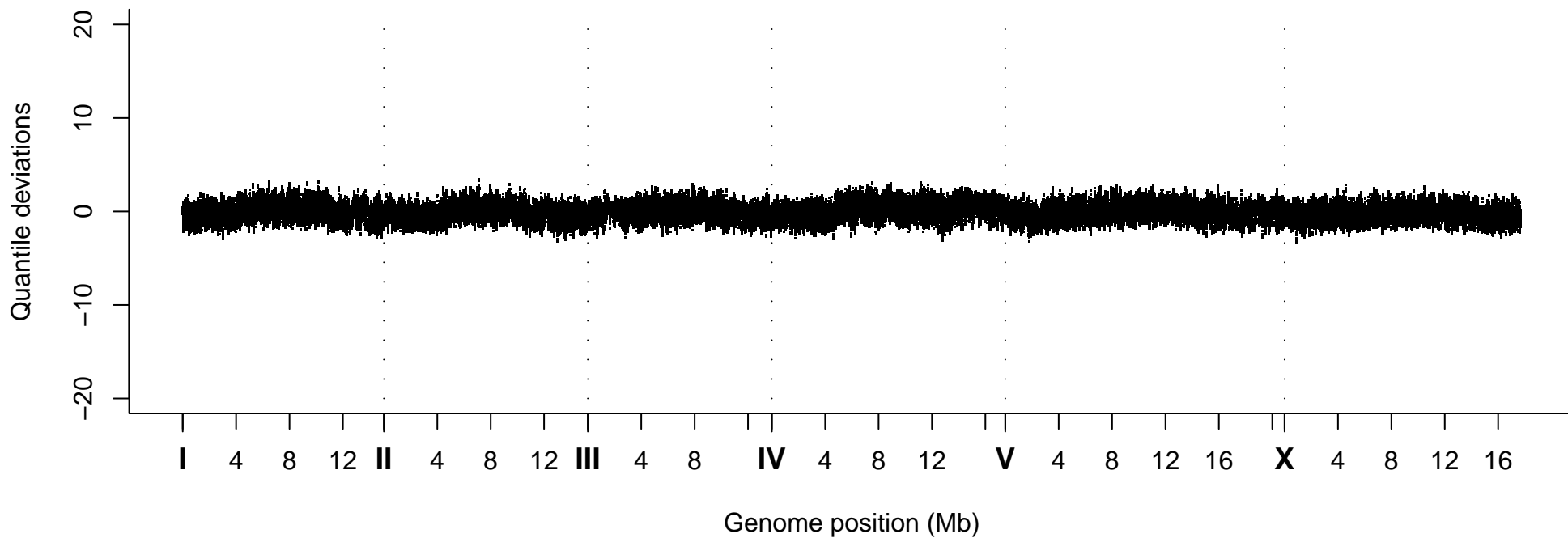
Quantile Deviations, Strain VC20492
