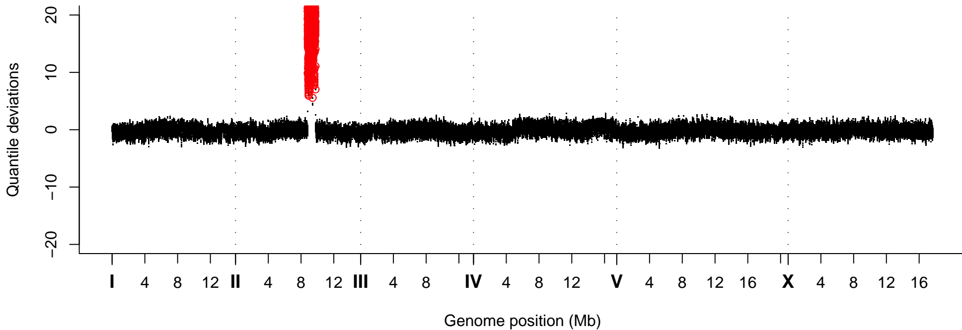
Quantile Deviations, Strain VC20499
