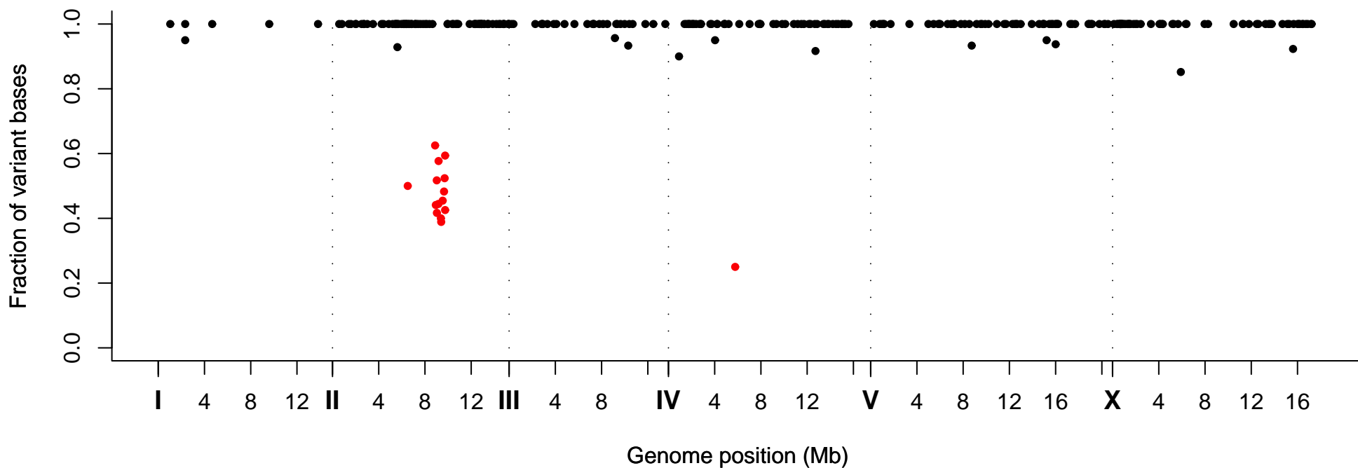
Fraction of Variant Bases at Position, Strain VC20499
