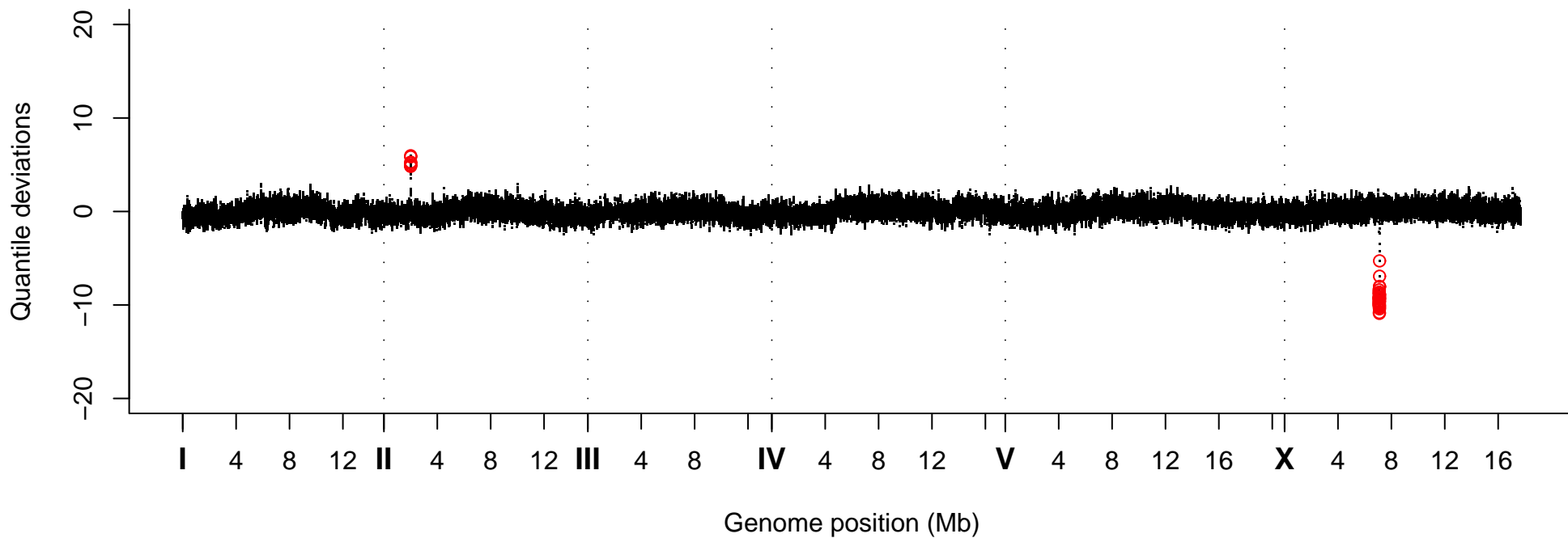
Quantile Deviations, Strain VC20503
