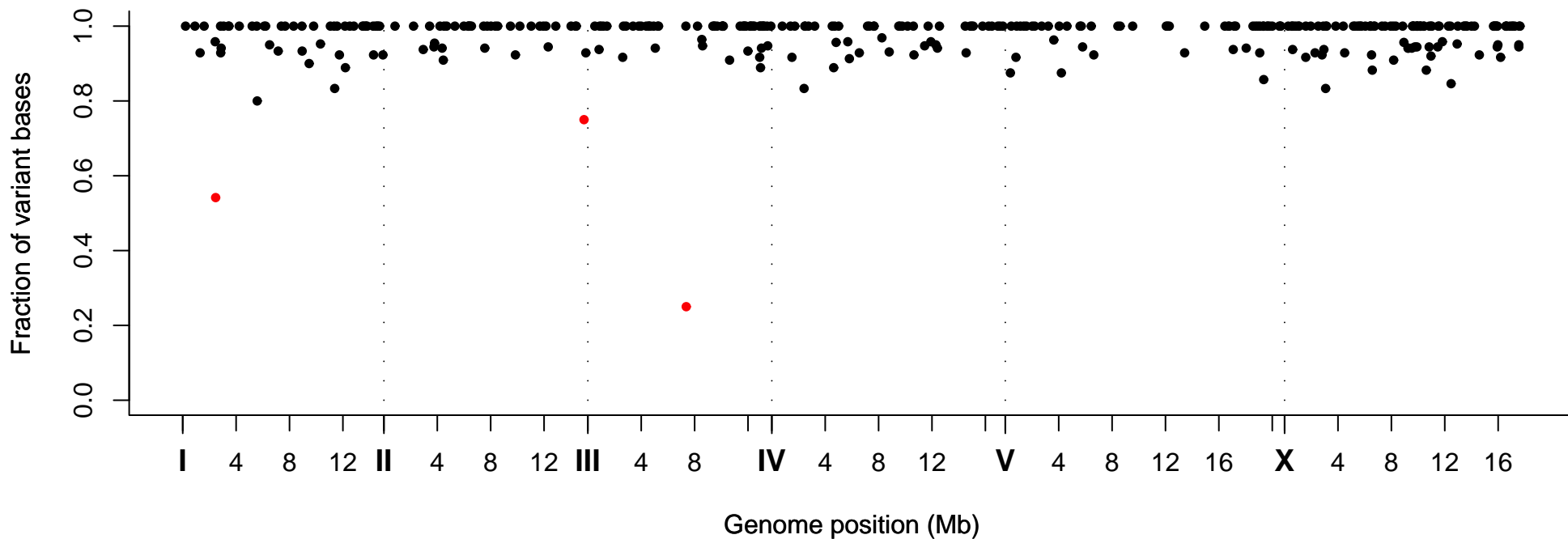
Fraction of Variant Bases at Position, Strain VC20503
