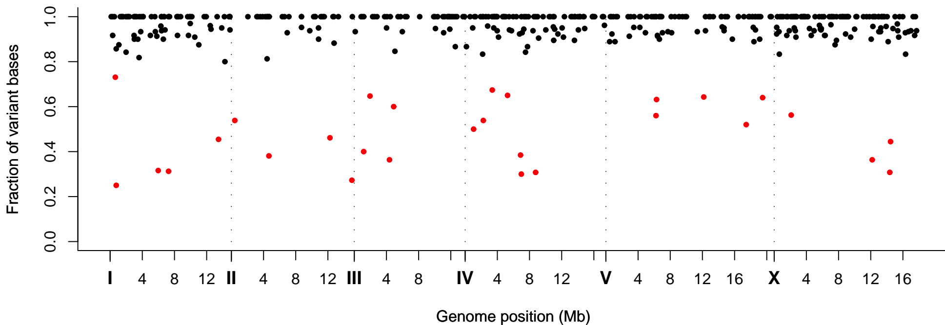
Fraction of Variant Bases at Position, Strain VC20507
