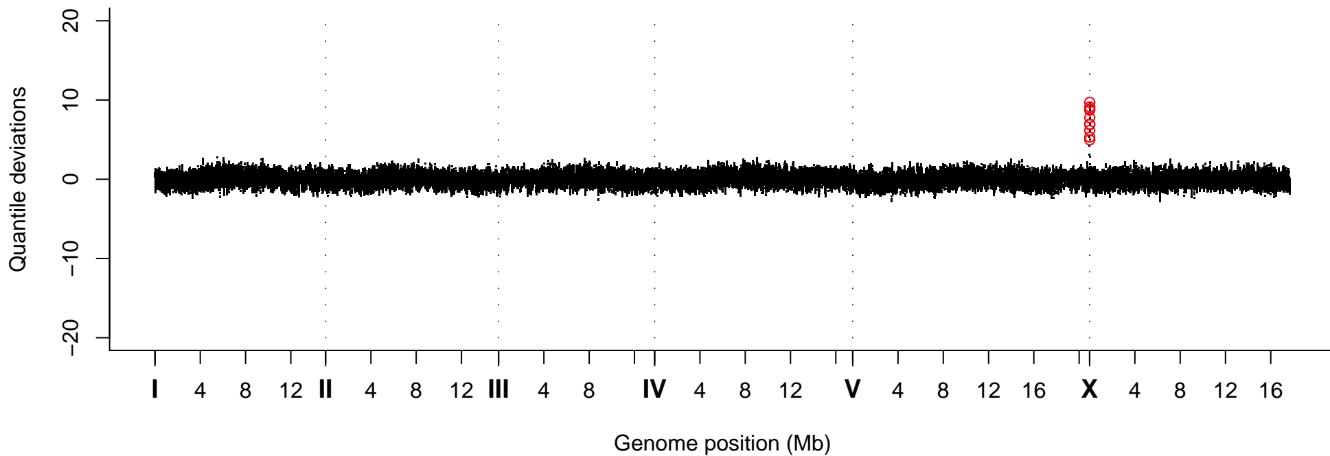
Quantile Deviations, Strain VC20507
