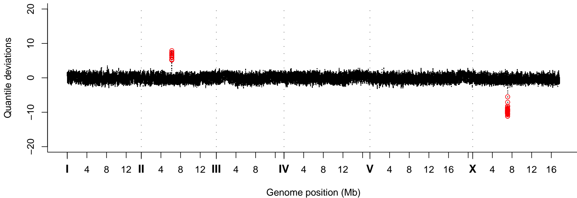
Quantile Deviations, Strain VC20512
