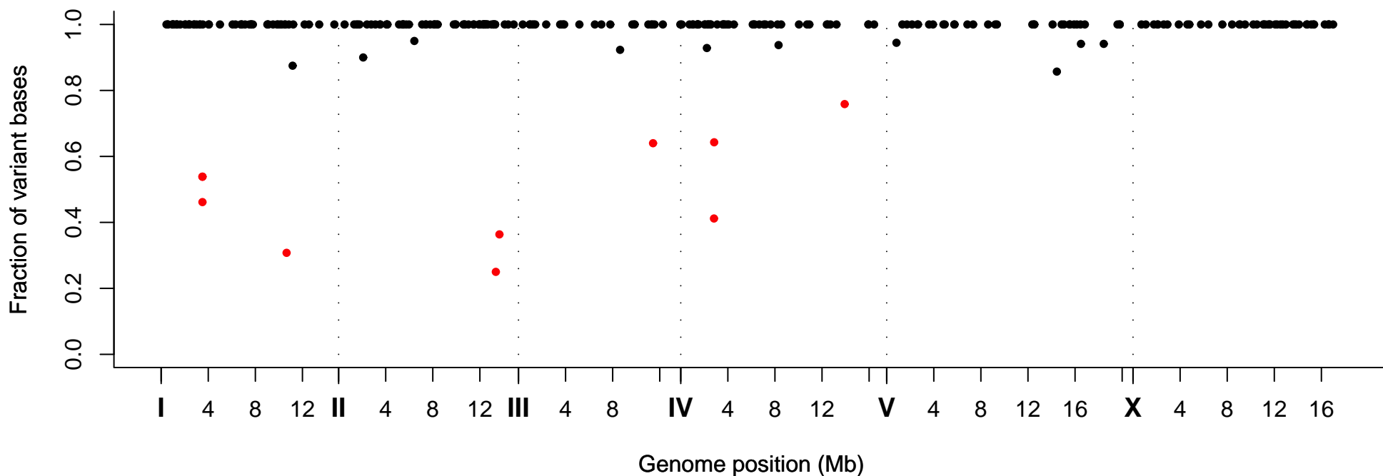
Fraction of Variant Bases at Position, Strain VC20512
