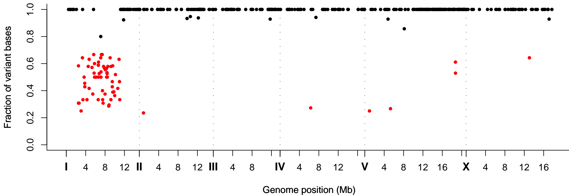
Fraction of Variant Bases at Position, Strain VC20523
