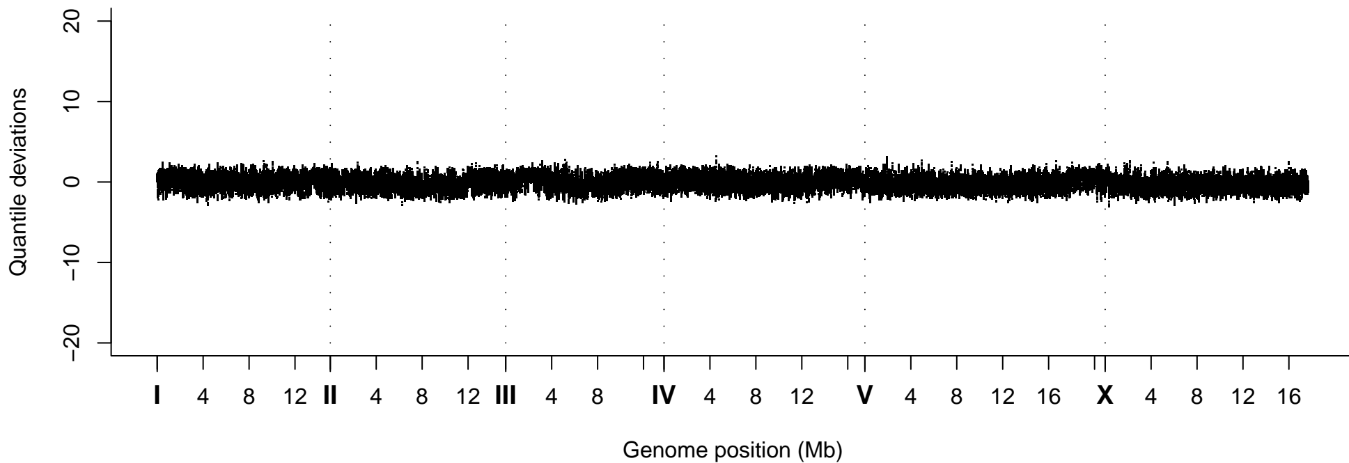
Quantile Deviations, Strain VC20523
