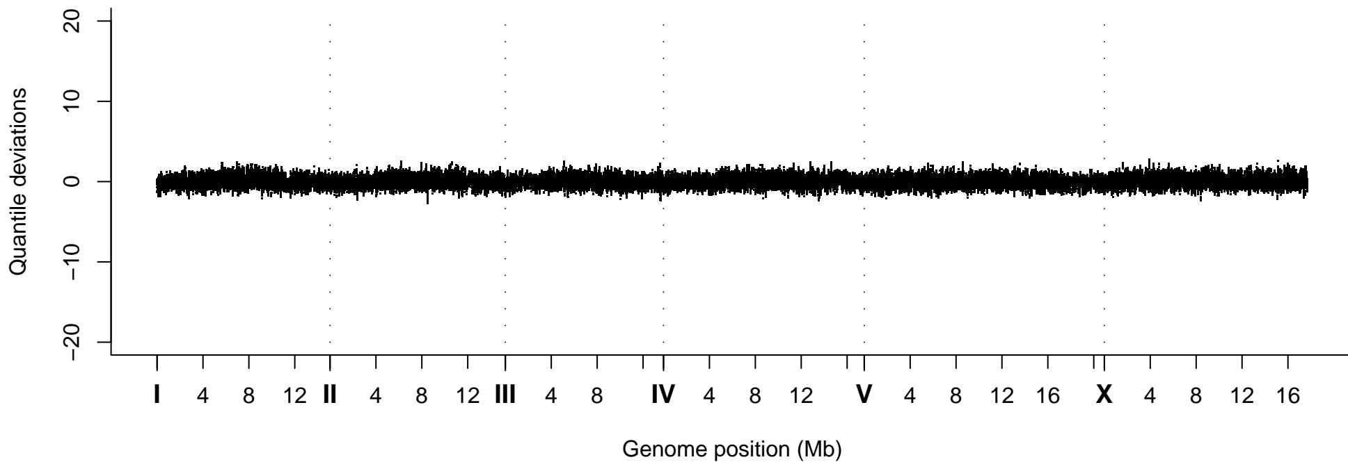
Quantile Deviations, Strain VC20531
