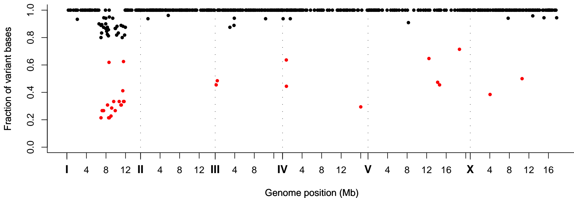
Fraction of Variant Bases at Position, Strain VC20531
