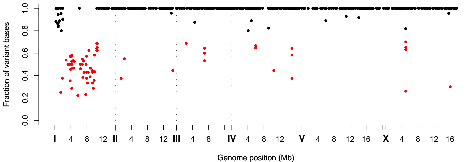
Fraction of Variant Bases at Position, Strain VC20536
