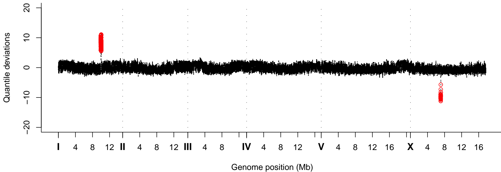
Quantile Deviations, Strain VC20536
