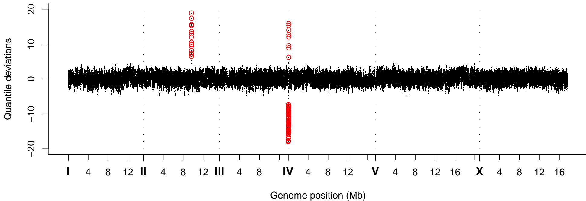
Quantile Deviations, Strain VC20537
