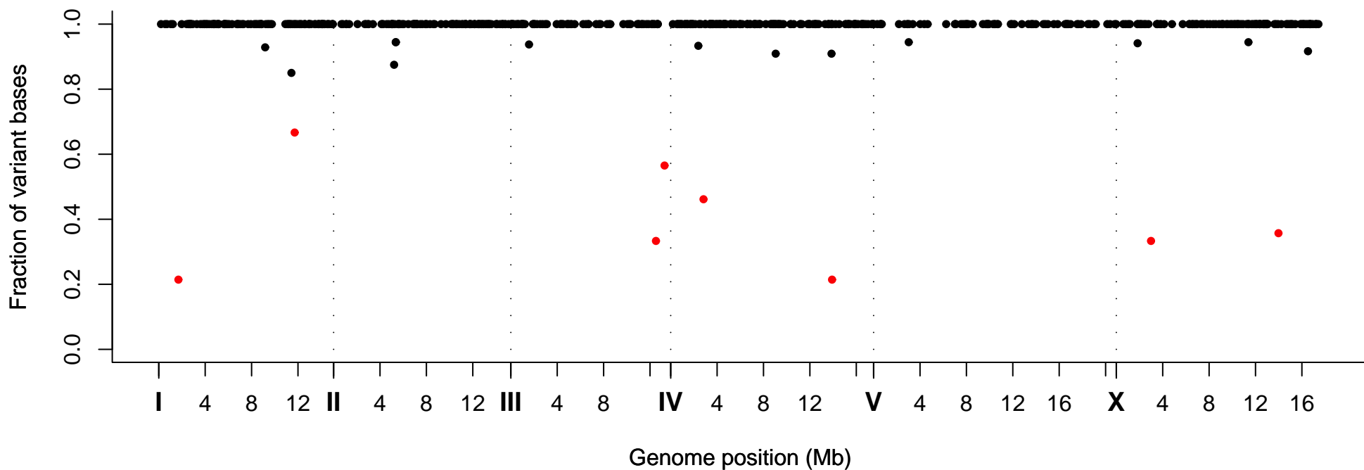
Fraction of Variant Bases at Position, Strain VC20537
