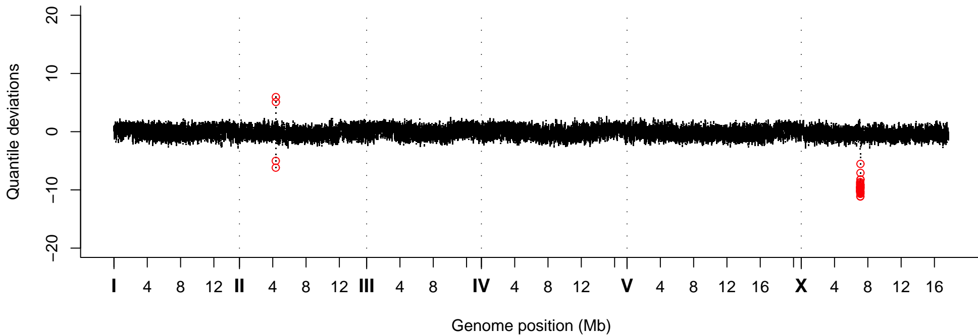
Quantile Deviations, Strain VC20540
