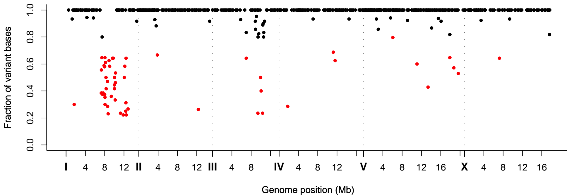
Fraction of Variant Bases at Position, Strain VC20540
