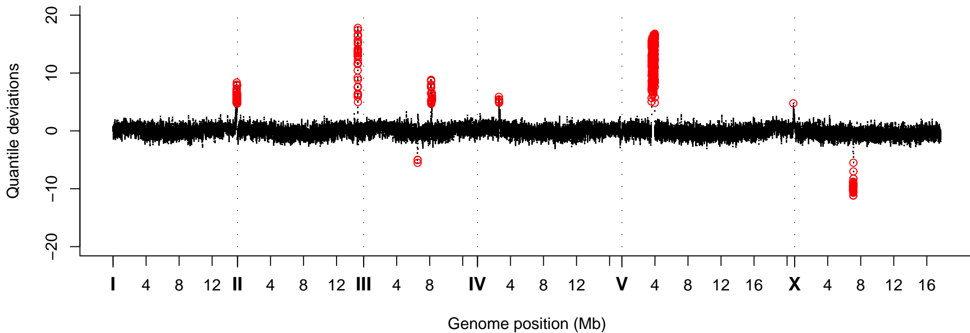
Quantile Deviations, Strain VC20542
