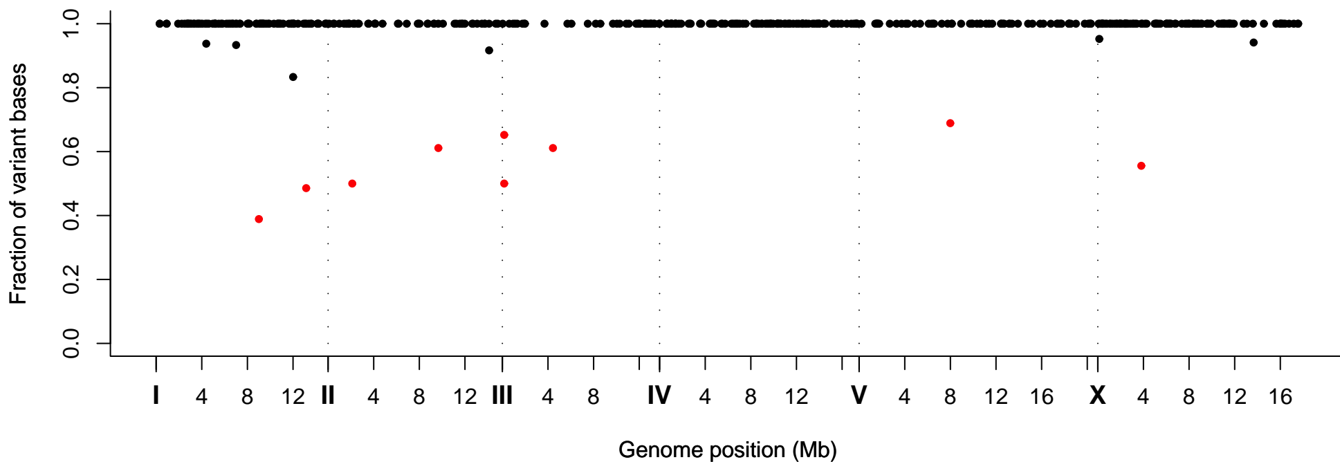
Fraction of Variant Bases at Position, Strain VC20544
