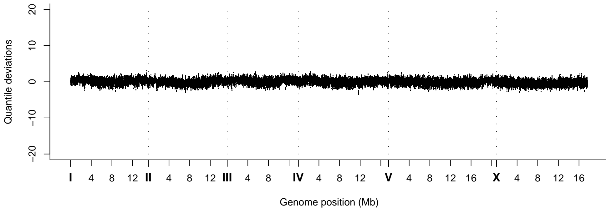
Quantile Deviations, Strain VC20544
