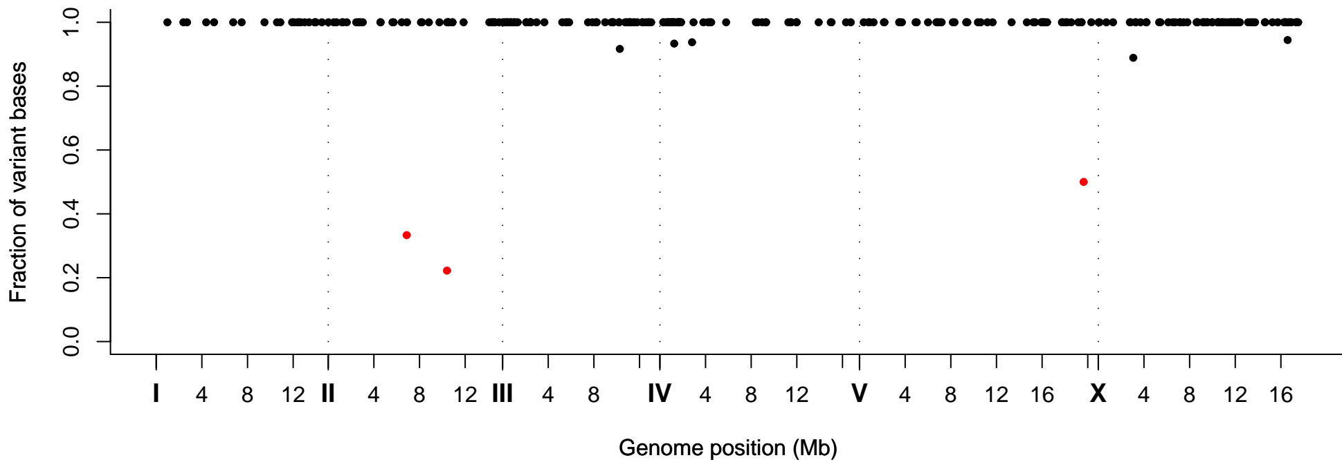
Fraction of Variant Bases at Position, Strain VC20566
