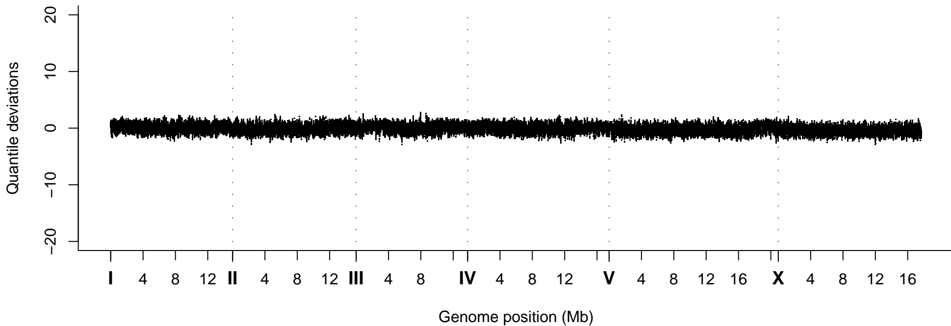
Quantile Deviations, Strain VC20566
