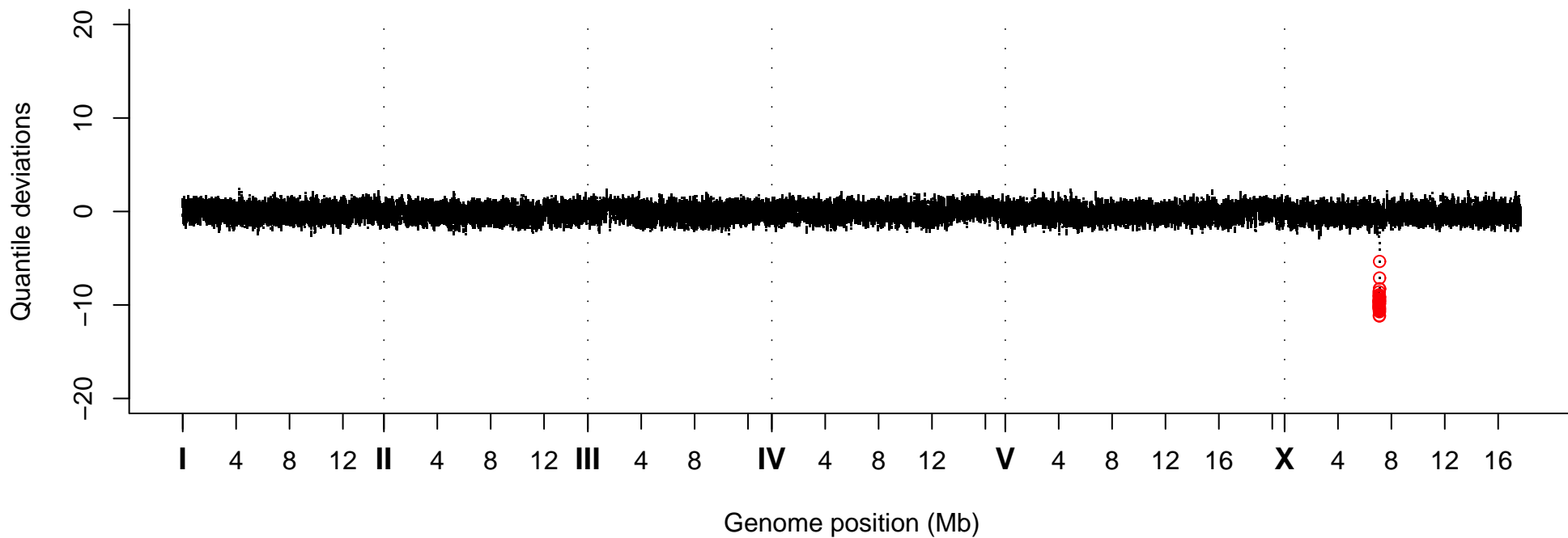
Quantile Deviations, Strain VC20567
