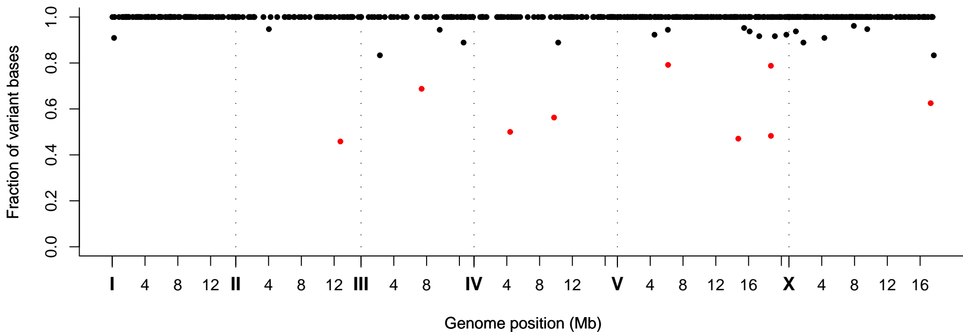
Fraction of Variant Bases at Position, Strain VC20567
