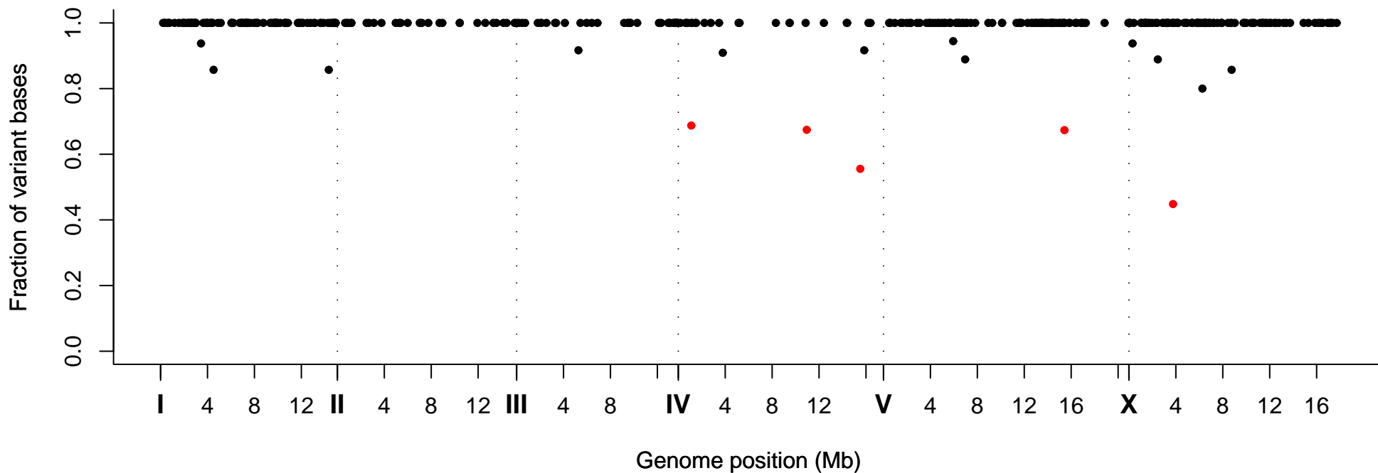
Fraction of Variant Bases at Position, Strain VC20571
