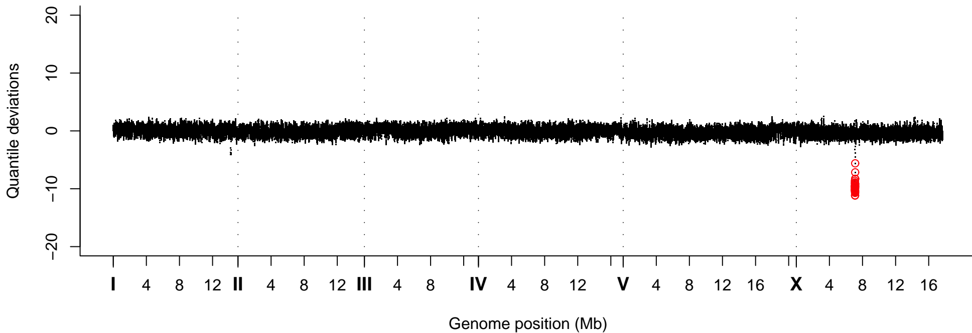
Quantile Deviations, Strain VC20571
