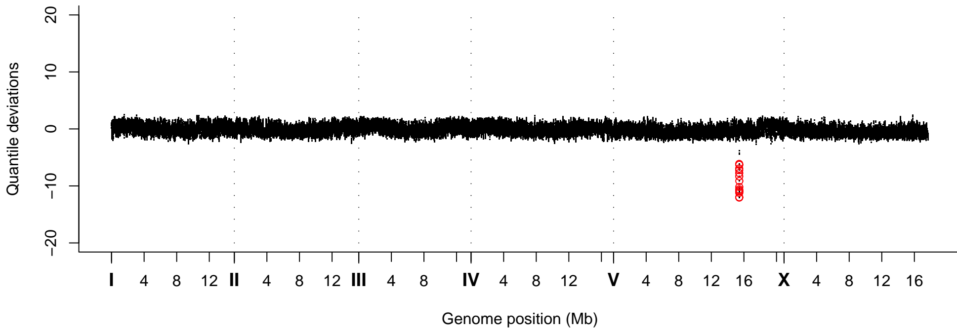
Quantile Deviations, Strain VC20580
