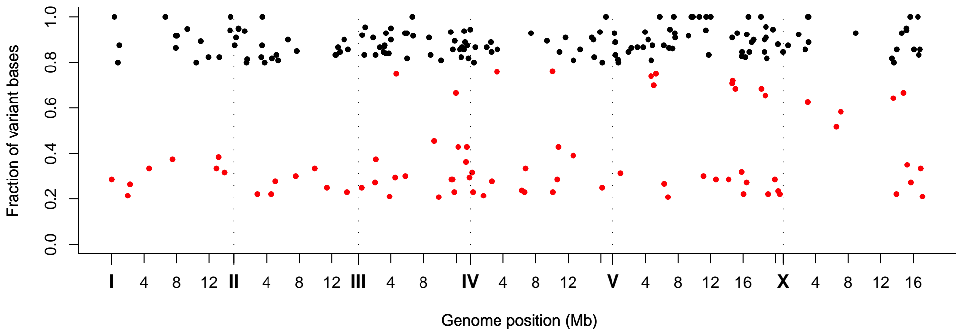
Fraction of Variant Bases at Position, Strain VC20580
