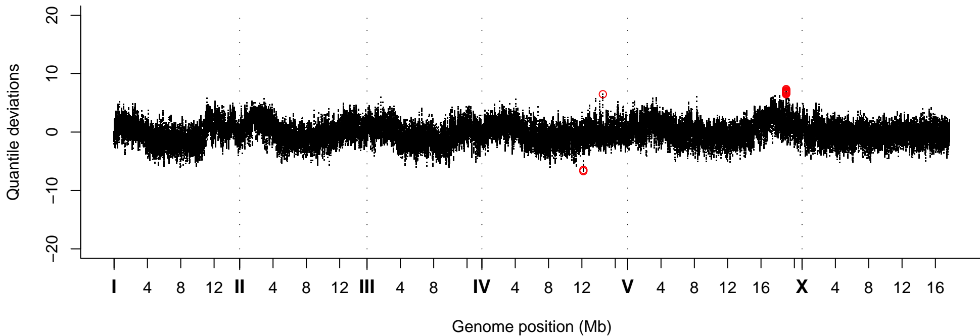
Quantile Deviations, Strain VC20582
