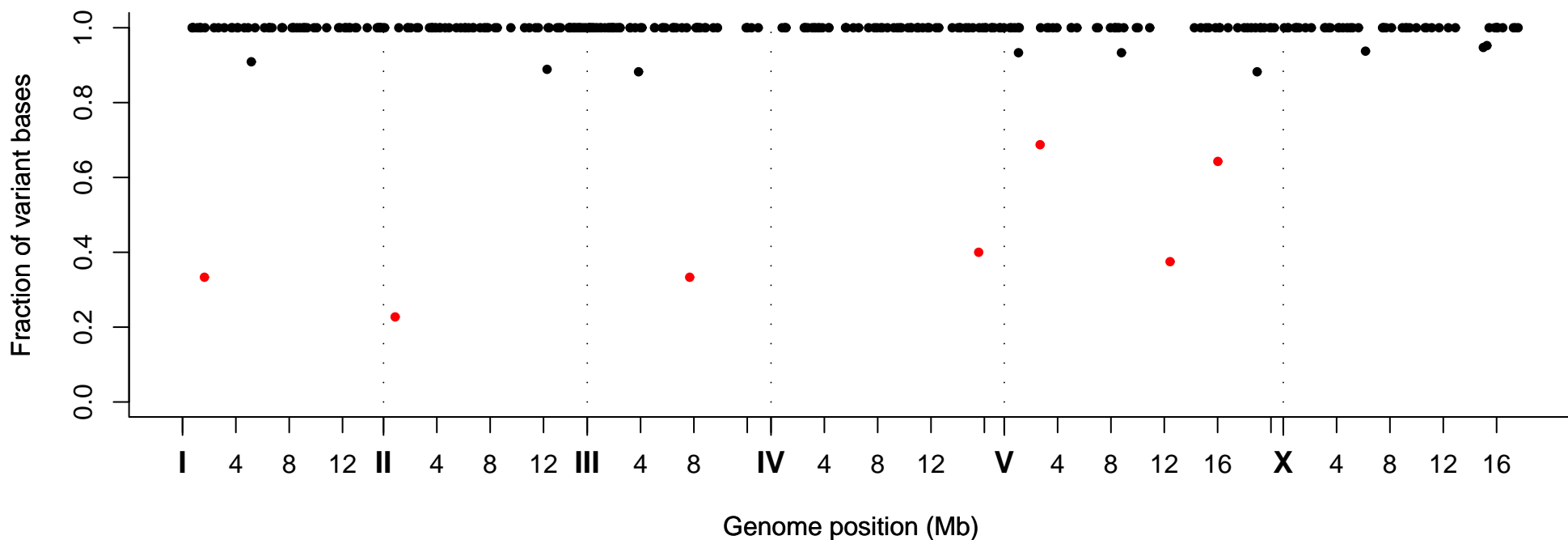
Fraction of Variant Bases at Position, Strain VC20582
