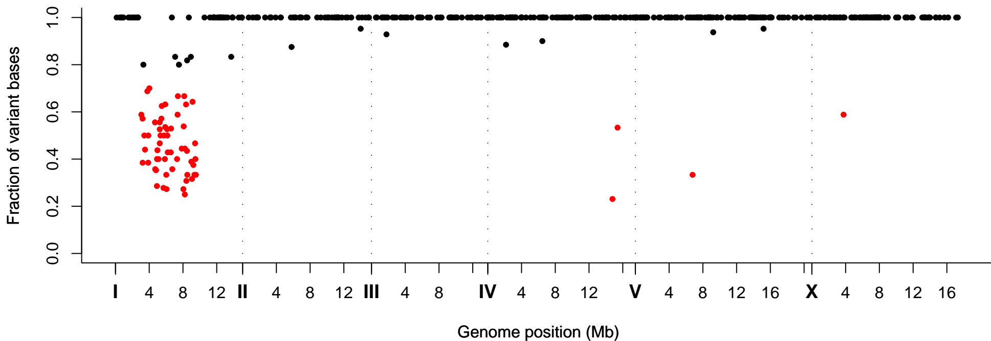
Fraction of Variant Bases at Position, Strain VC20585
