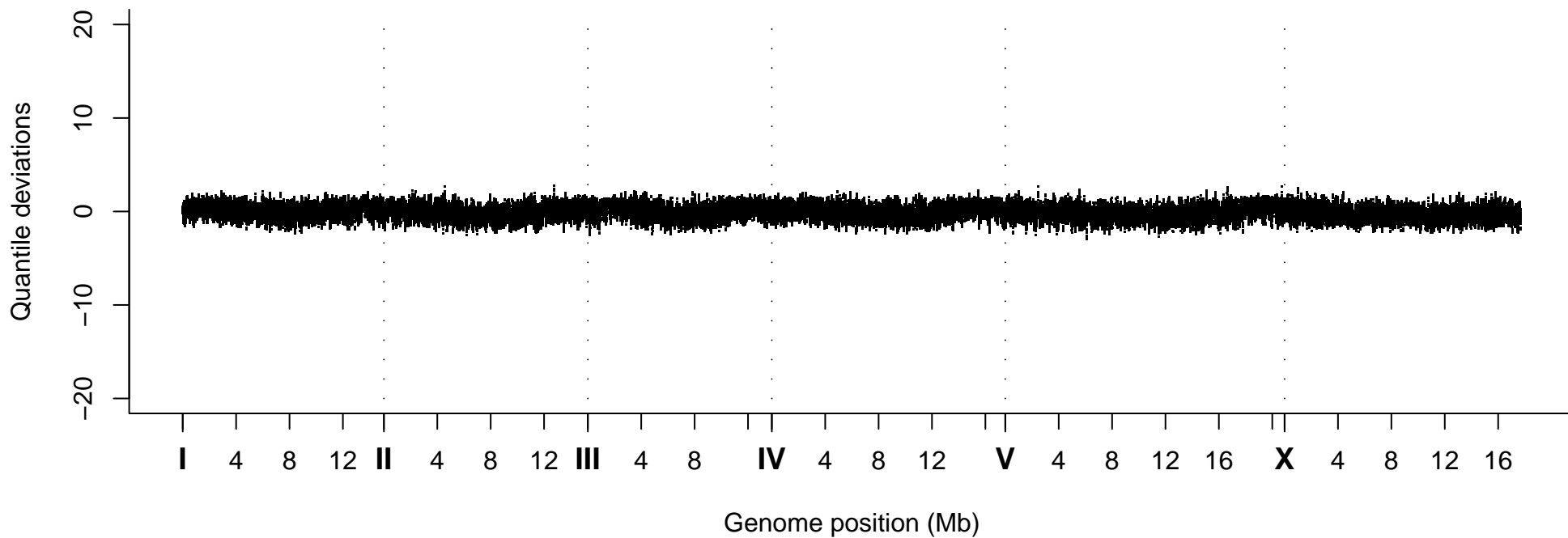
Quantile Deviations, Strain VC20585
