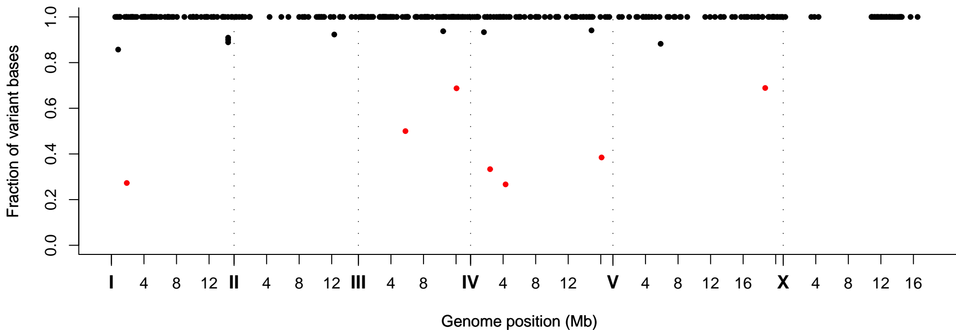
Fraction of Variant Bases at Position, Strain VC20586
