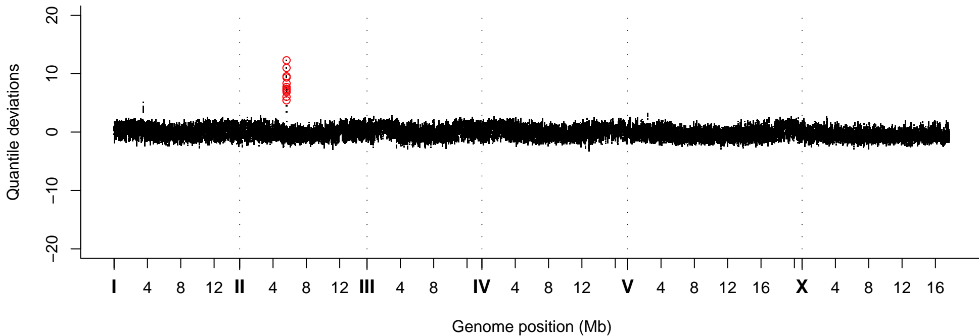
Quantile Deviations, Strain VC20586
