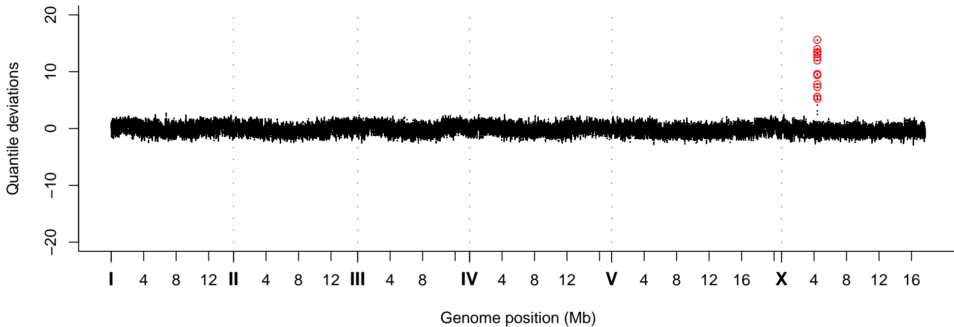
Quantile Deviations, Strain VC20587
