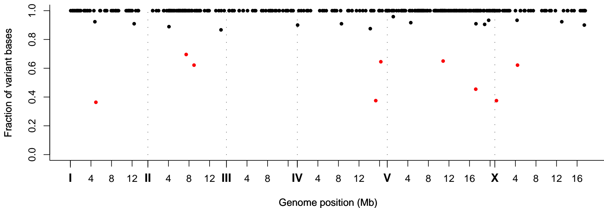
Fraction of Variant Bases at Position, Strain VC20587
