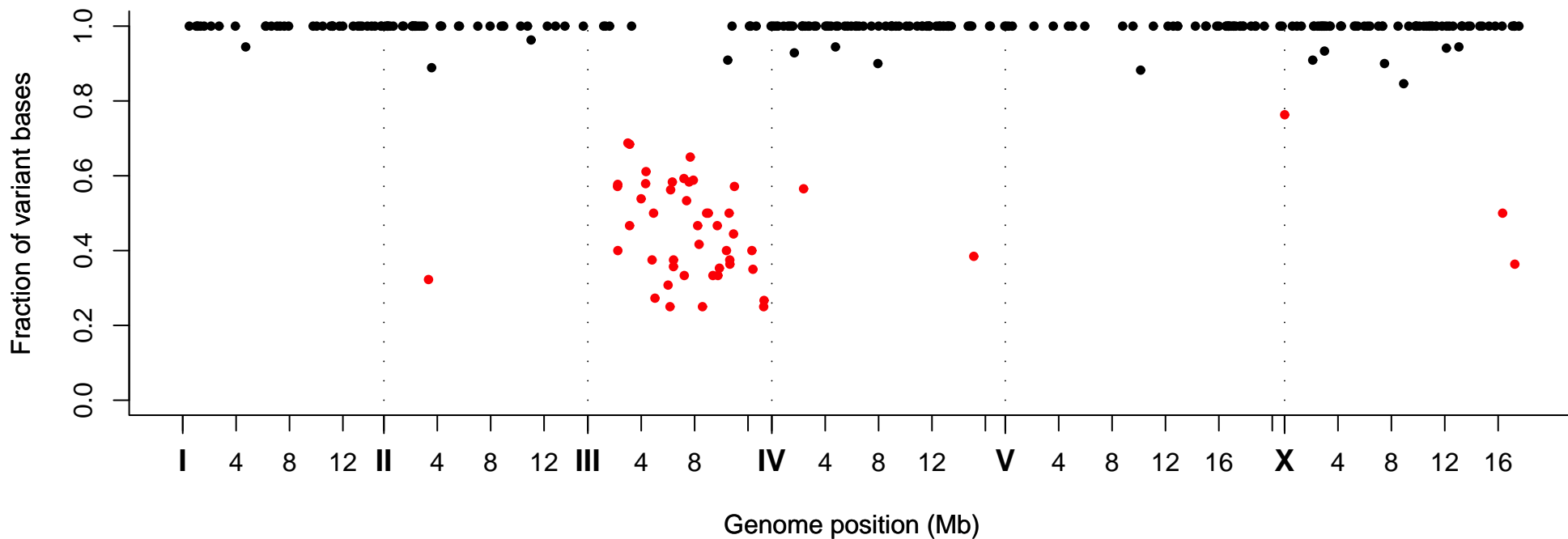
Fraction of Variant Bases at Position, Strain VC20593
