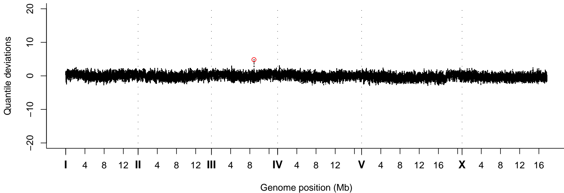
Quantile Deviations, Strain VC20593
