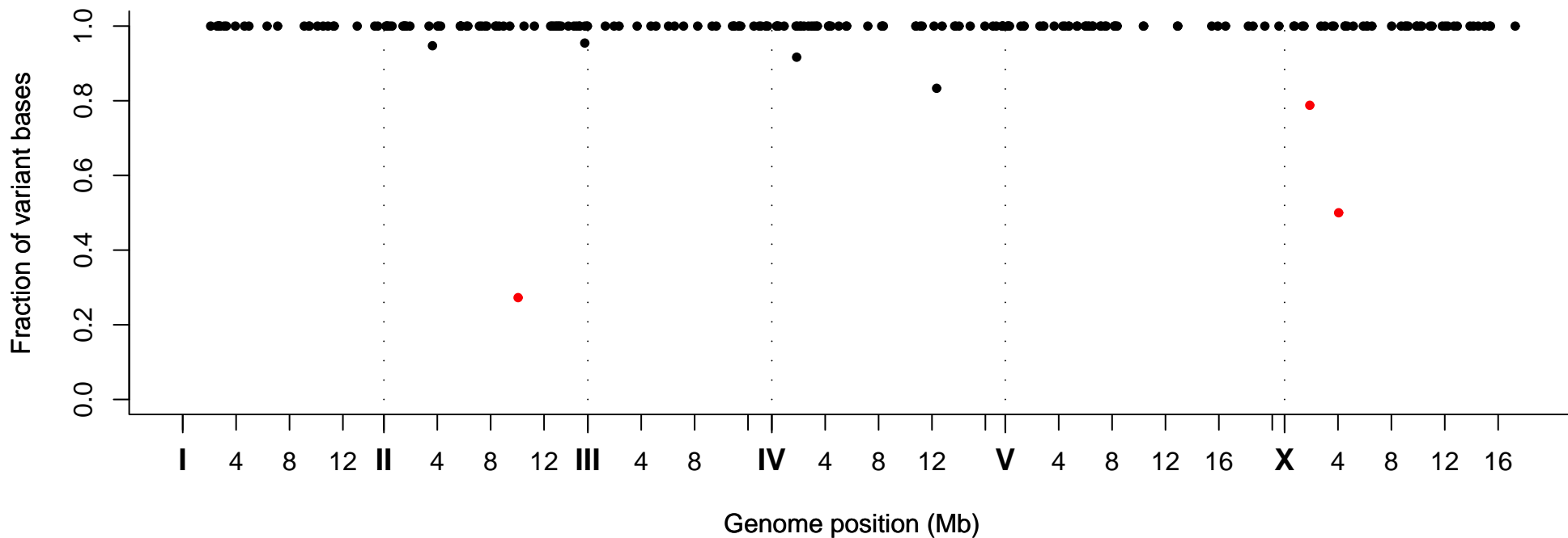
Fraction of Variant Bases at Position, Strain VC20594
