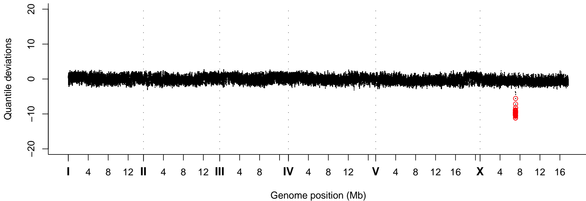
Quantile Deviations, Strain VC20594
