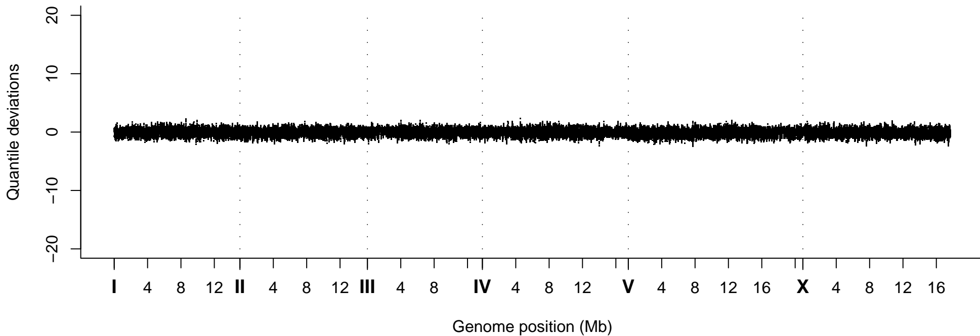
Quantile Deviations, Strain VC20604
