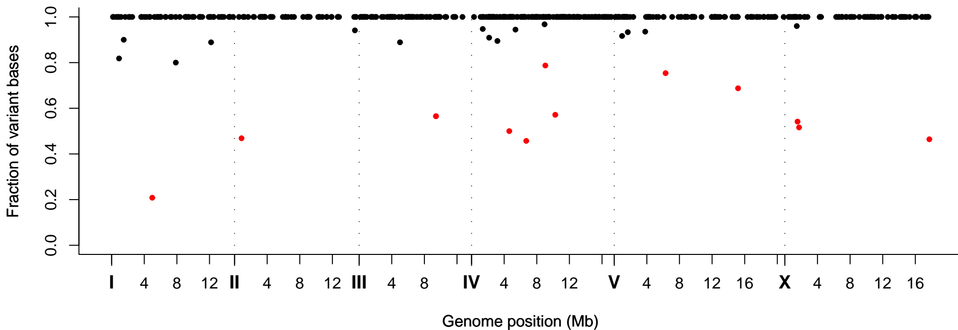
Fraction of Variant Bases at Position, Strain VC20604
