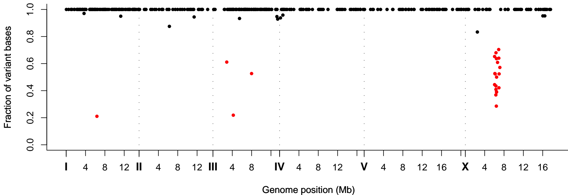
Fraction of Variant Bases at Position, Strain VC20607
