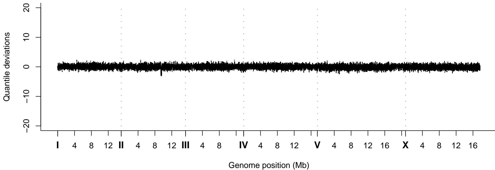
Quantile Deviations, Strain VC20607
