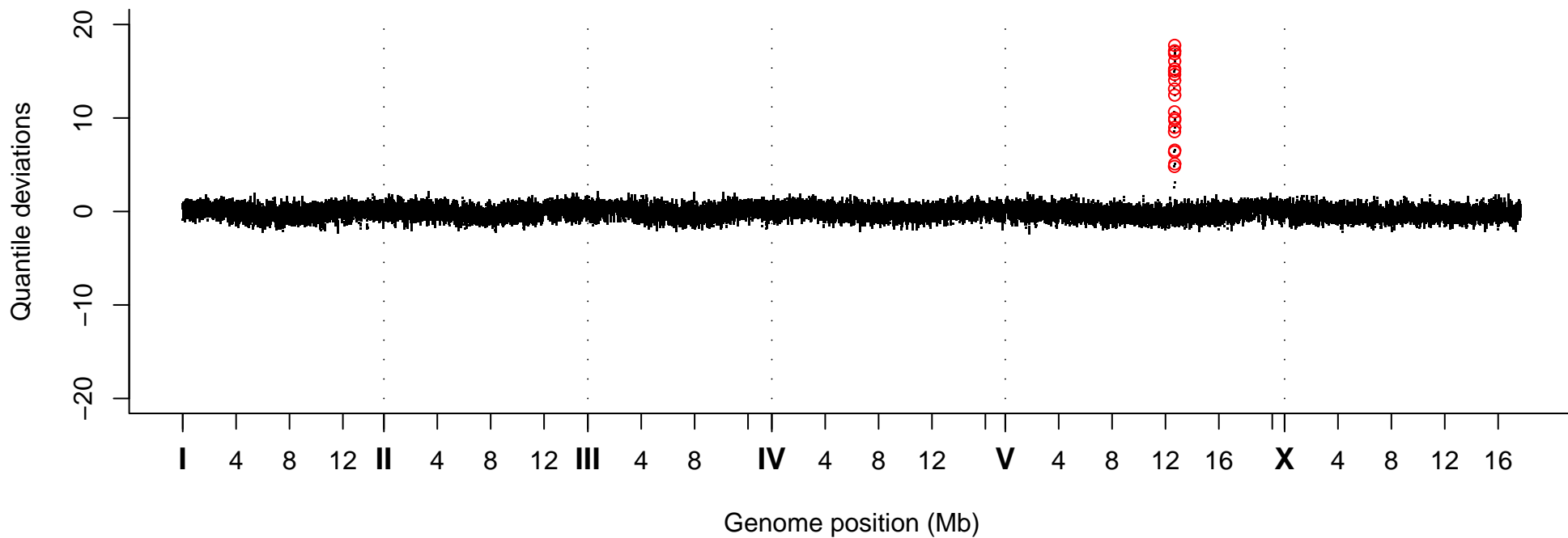
Quantile Deviations, Strain VC20608
