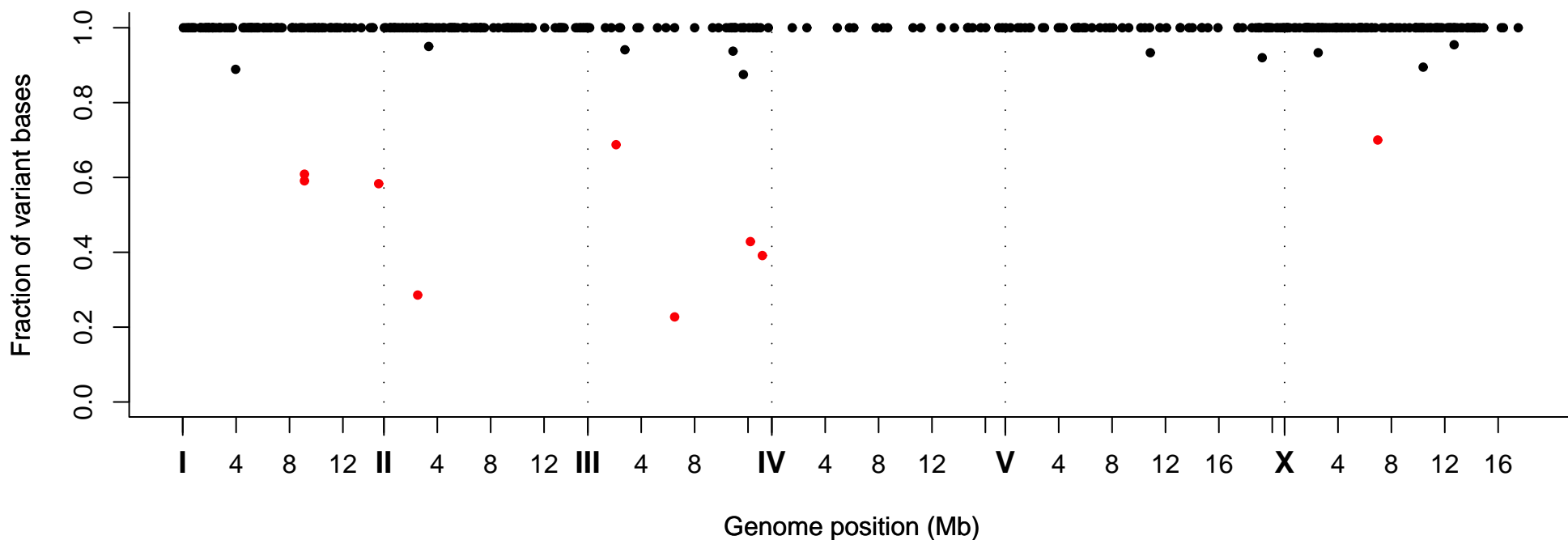
Fraction of Variant Bases at Position, Strain VC20608
