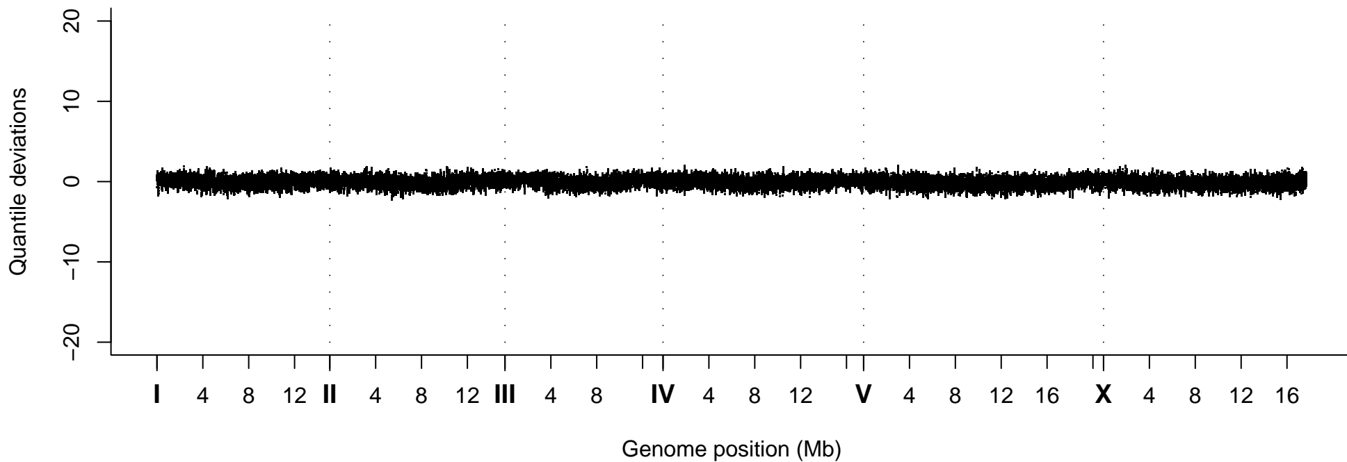
Quantile Deviations, Strain VC20609
