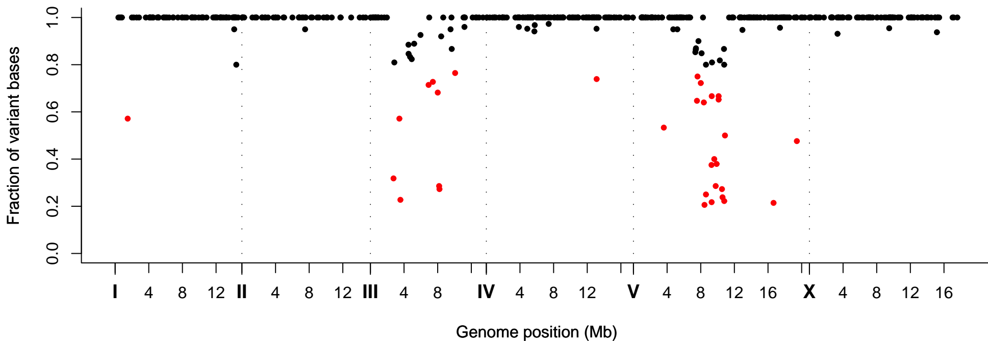
Fraction of Variant Bases at Position, Strain VC20609
