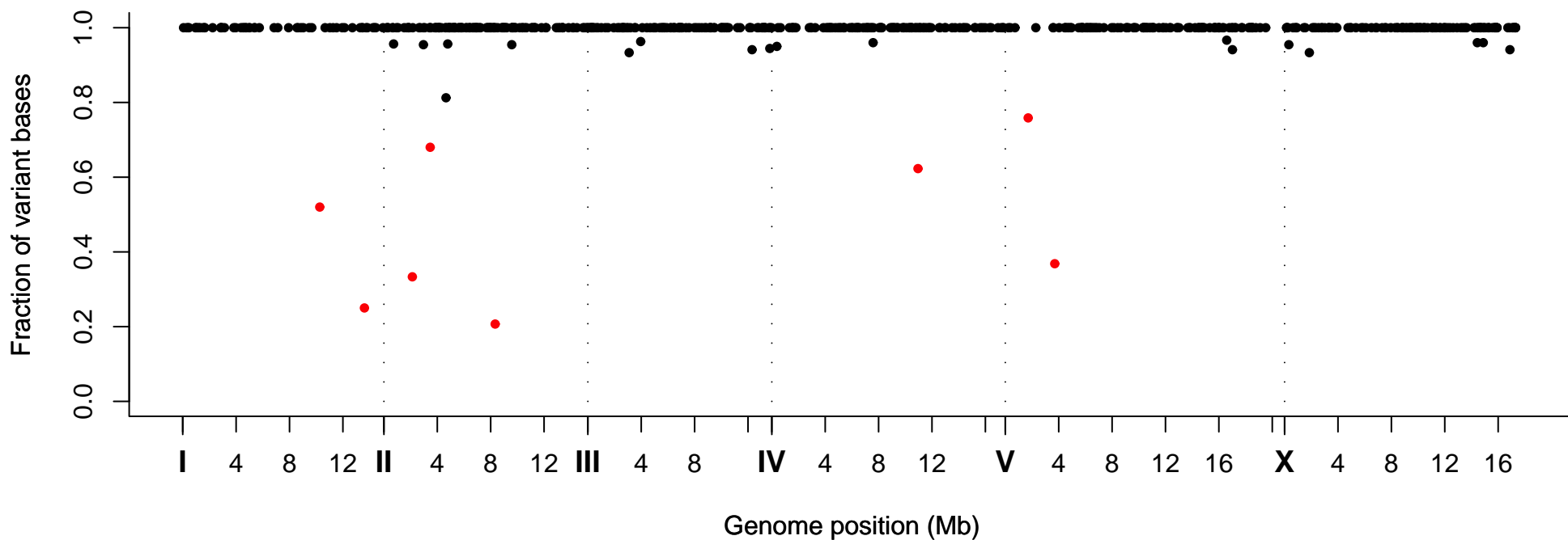
Fraction of Variant Bases at Position, Strain VC20610
