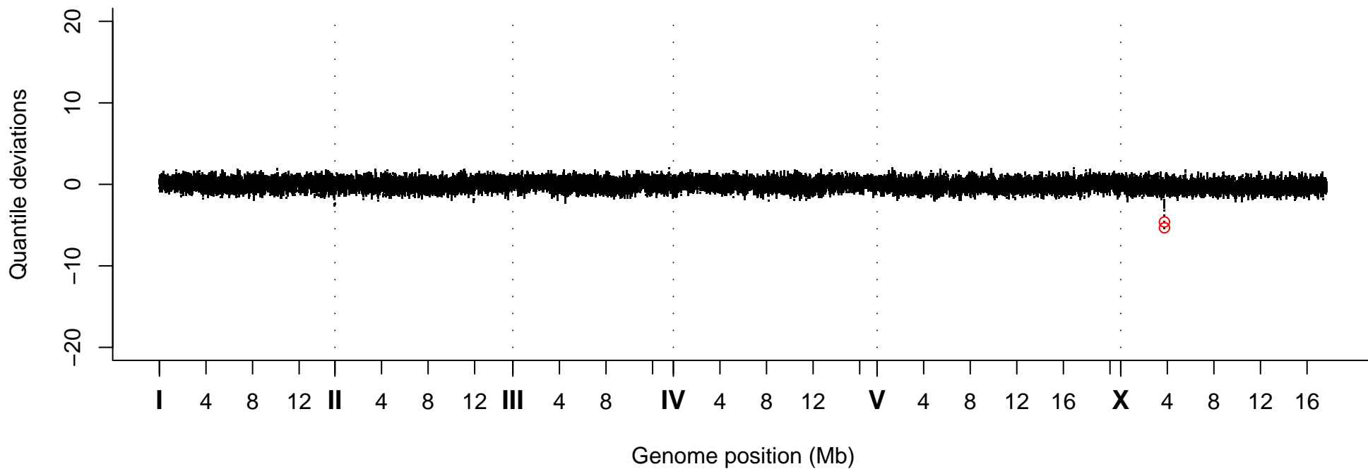
Quantile Deviations, Strain VC20610
