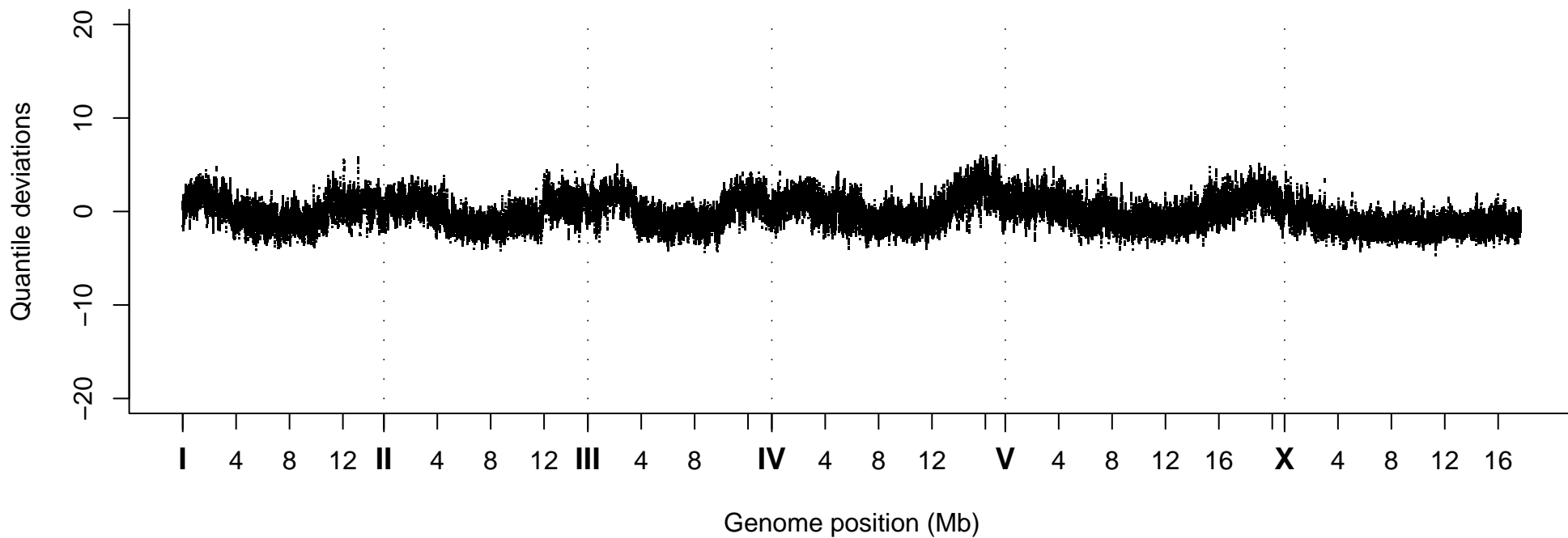
Quantile Deviations, Strain VC20611
