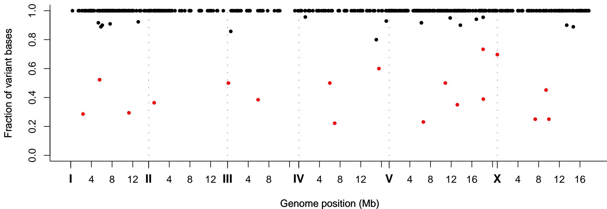
Fraction of Variant Bases at Position, Strain VC20611
