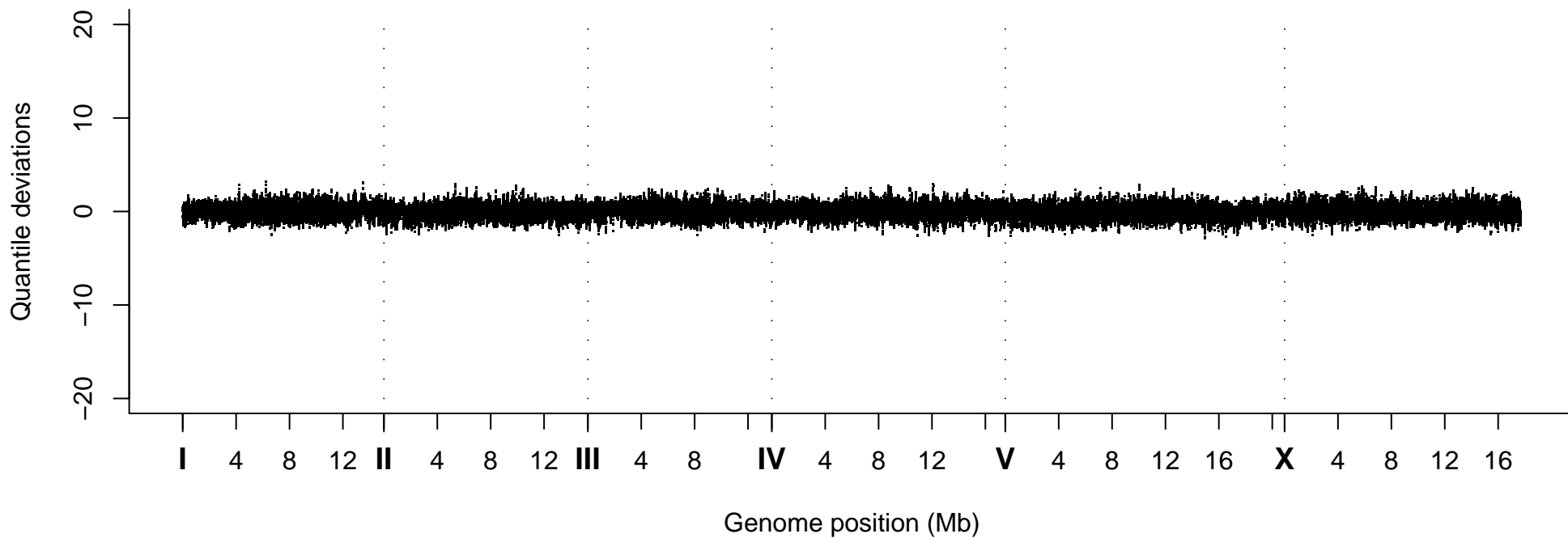
Quantile Deviations, Strain VC20618
