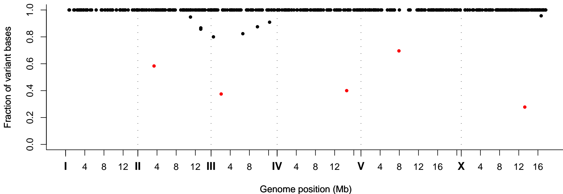
Fraction of Variant Bases at Position, Strain VC20618
