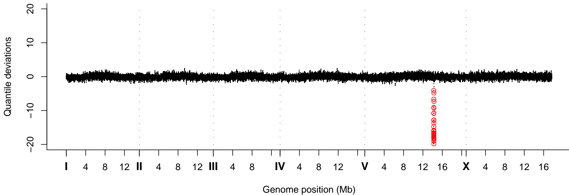
Quantile Deviations, Strain VC20619
