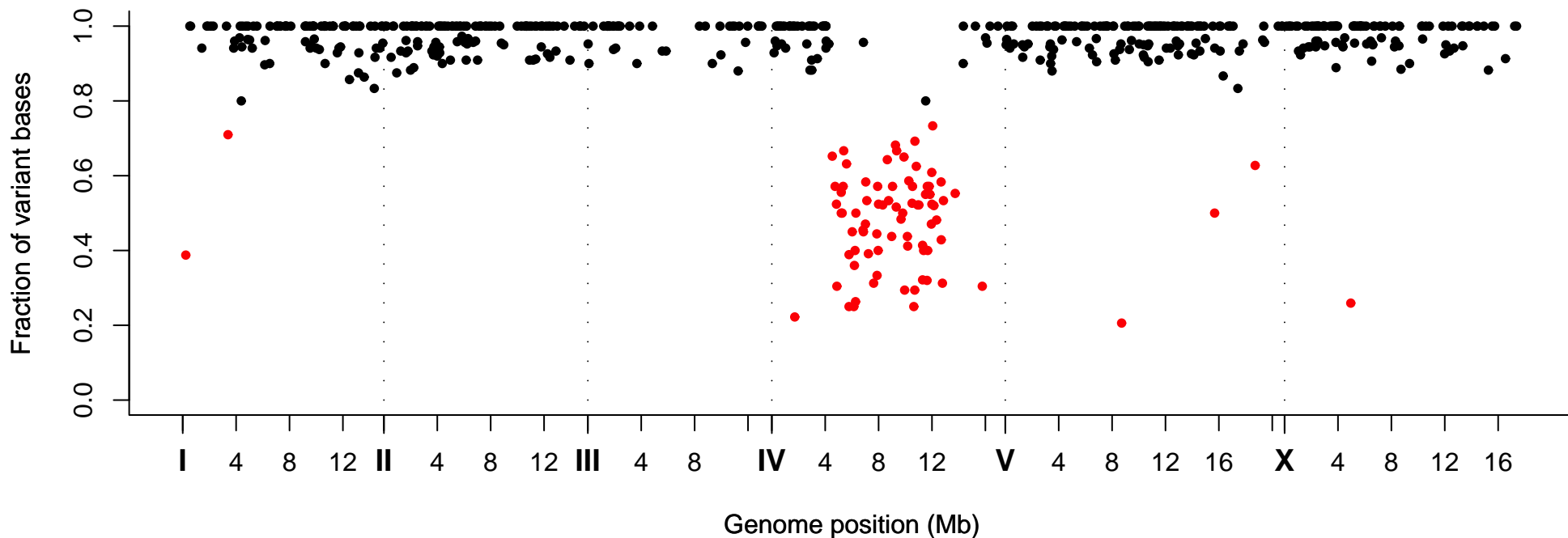
Fraction of Variant Bases at Position, Strain VC20619
