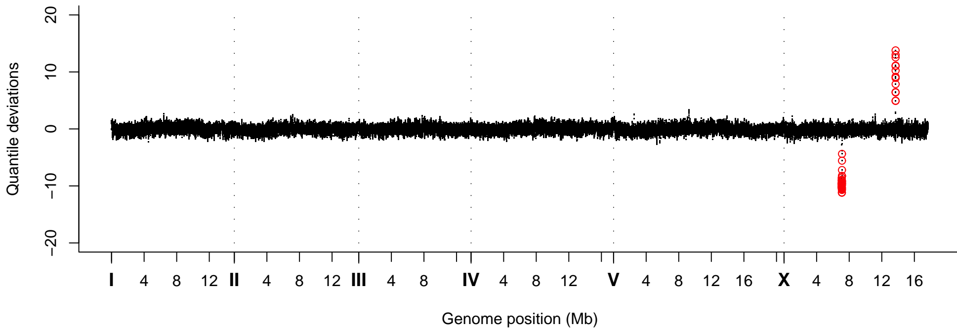
Quantile Deviations, Strain VC20625
