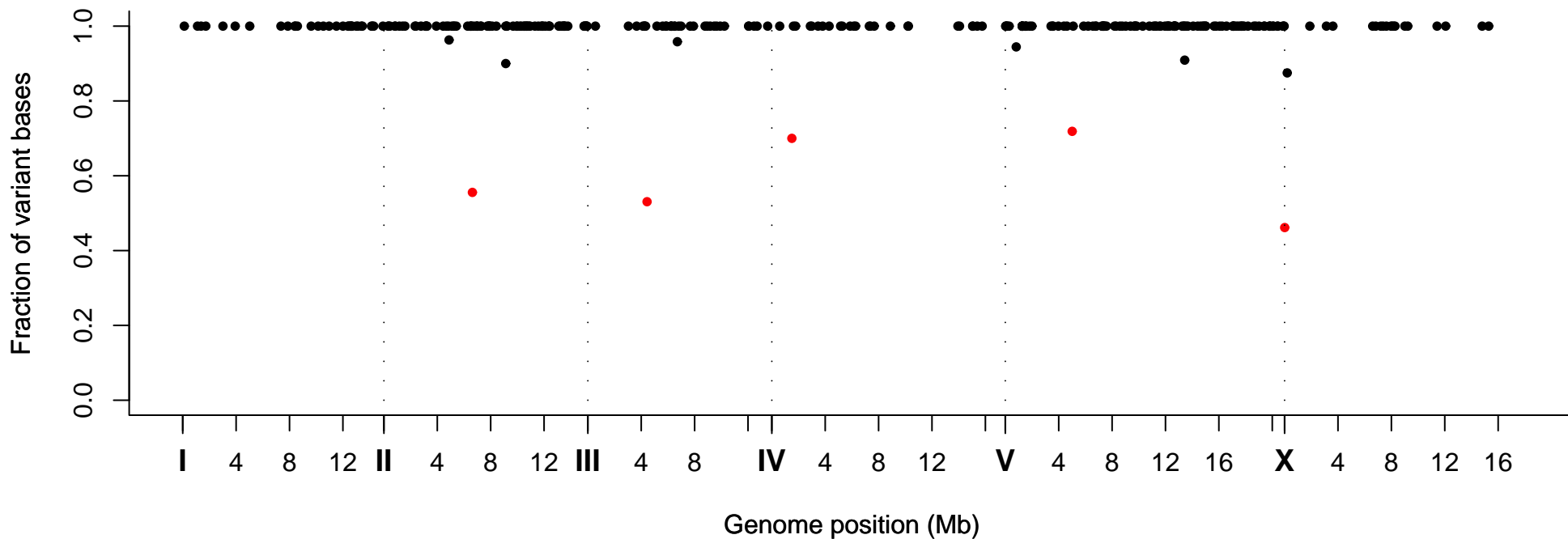
Fraction of Variant Bases at Position, Strain VC20625
