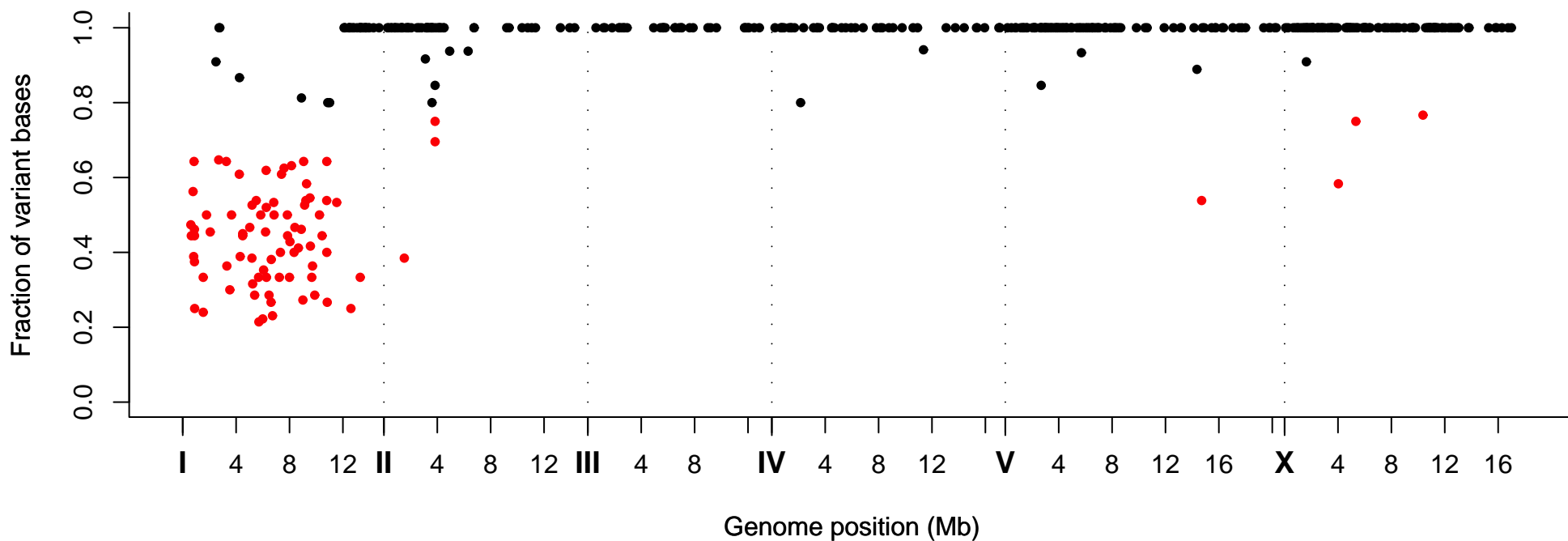
Fraction of Variant Bases at Position, Strain VC20633
