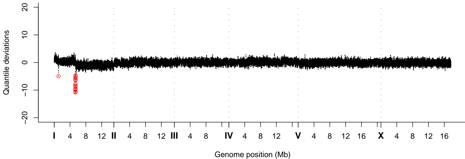
Quantile Deviations, Strain VC20633
