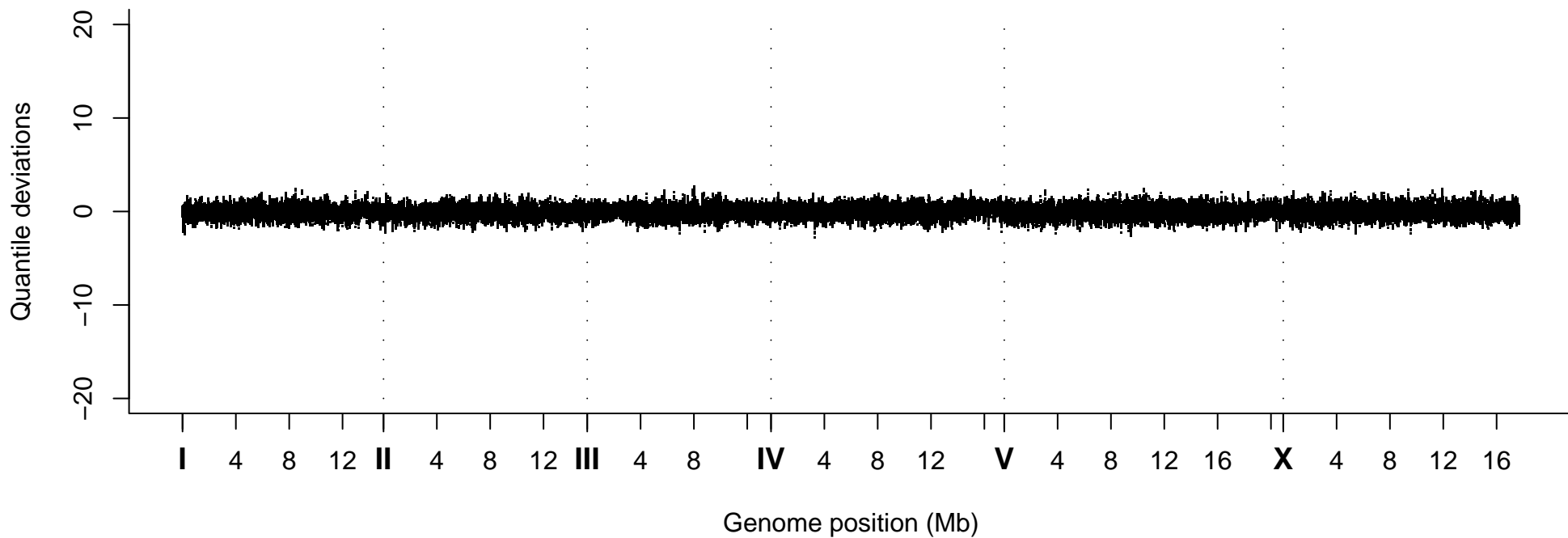
Quantile Deviations, Strain VC20634
