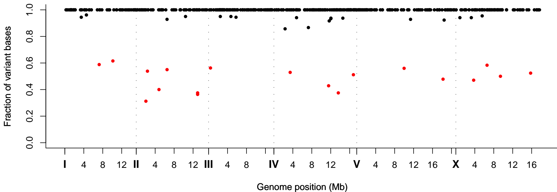
Fraction of Variant Bases at Position, Strain VC20634
