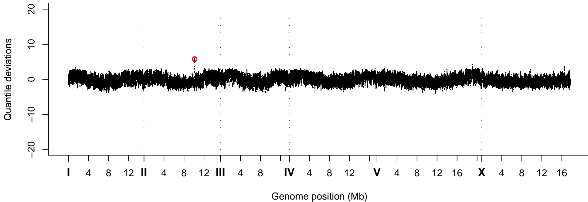
Quantile Deviations, Strain VC20648
