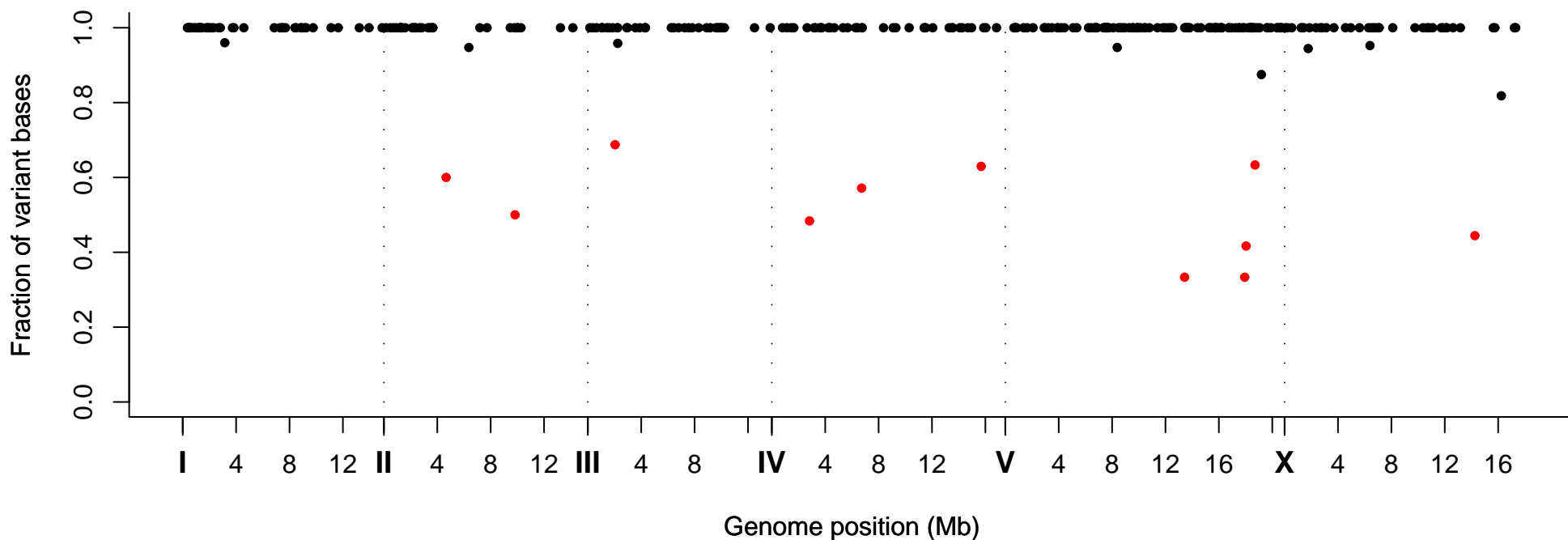
Fraction of Variant Bases at Position, Strain VC20648
