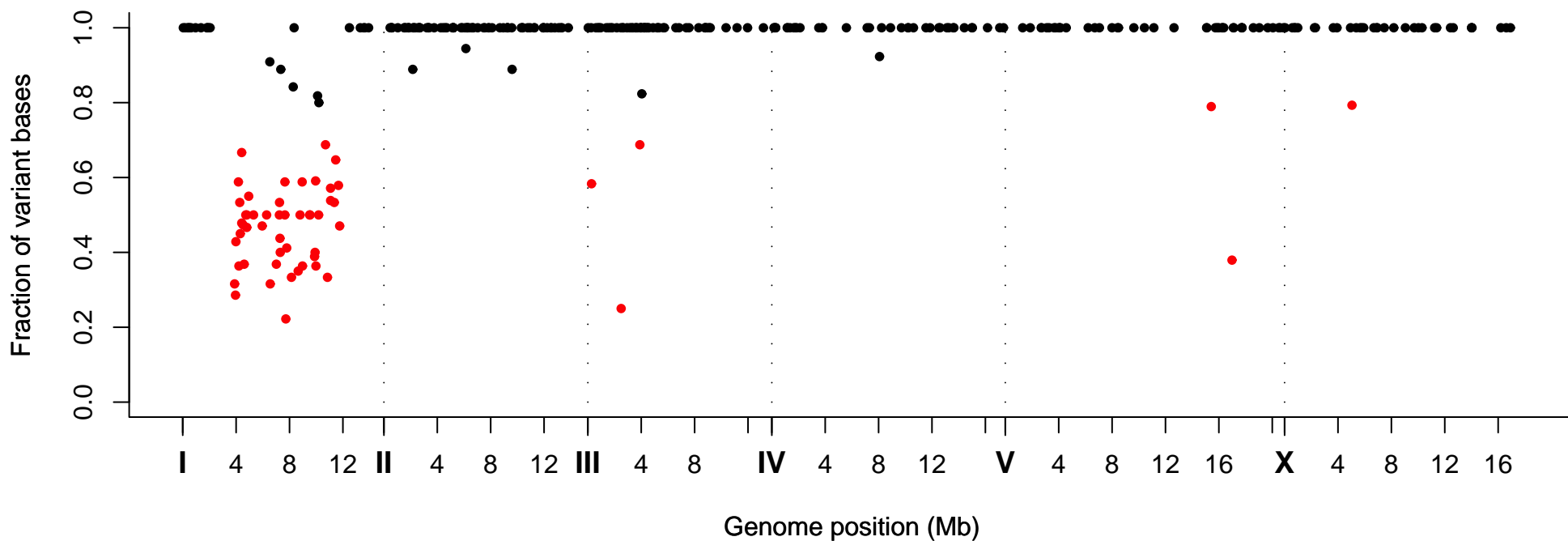
Fraction of Variant Bases at Position, Strain VC20649
