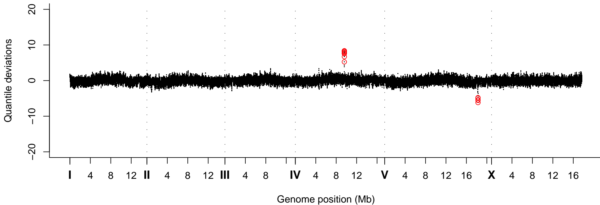
Quantile Deviations, Strain VC20649
