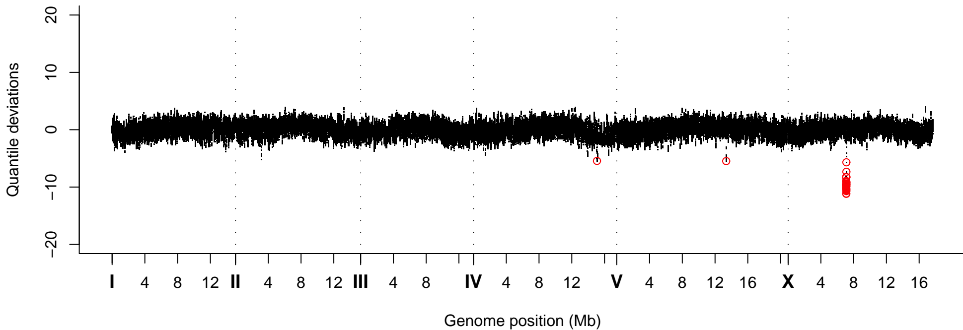
Quantile Deviations, Strain VC20671
