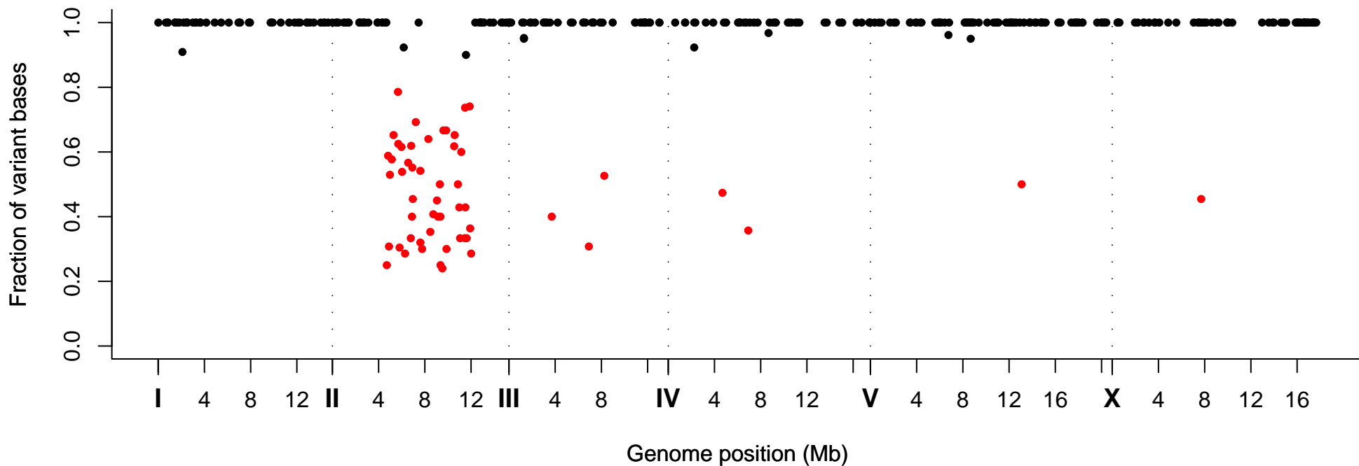
Fraction of Variant Bases at Position, Strain VC20671
