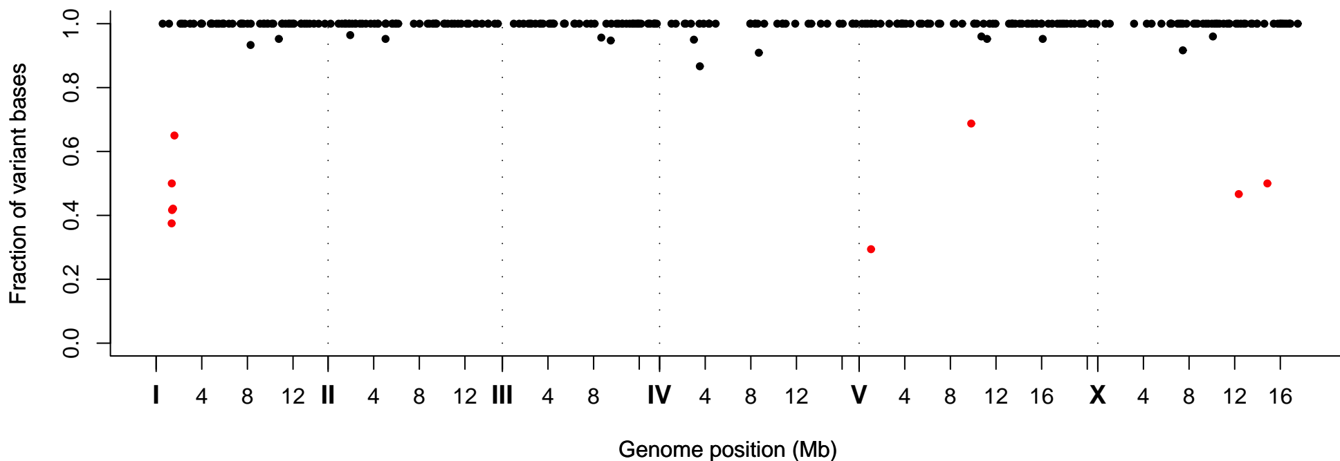
Fraction of Variant Bases at Position, Strain VC20678
