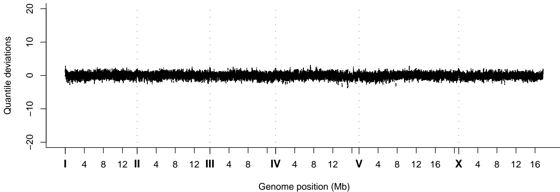
Quantile Deviations, Strain VC20678
